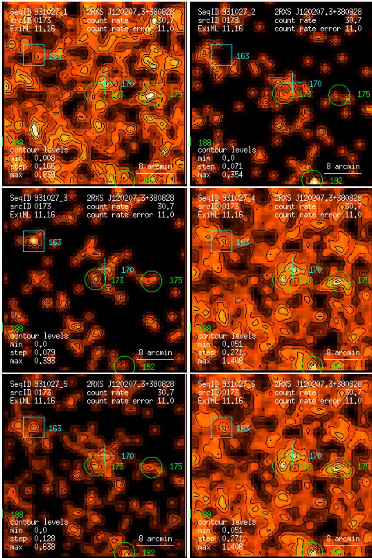
Figure 173: RASS 931027: detection 0173: band rate images, Gaussian filter: (1) PSPC channels 11 – 41, (2) 52 – 90, (3) 91 – 201, (4) 11 – 235, (5) 52 – 201, (6) 11 – 201. Broad band rates in counts/ks. Band rate contour levels in counts/ks/arcmin 2 .
