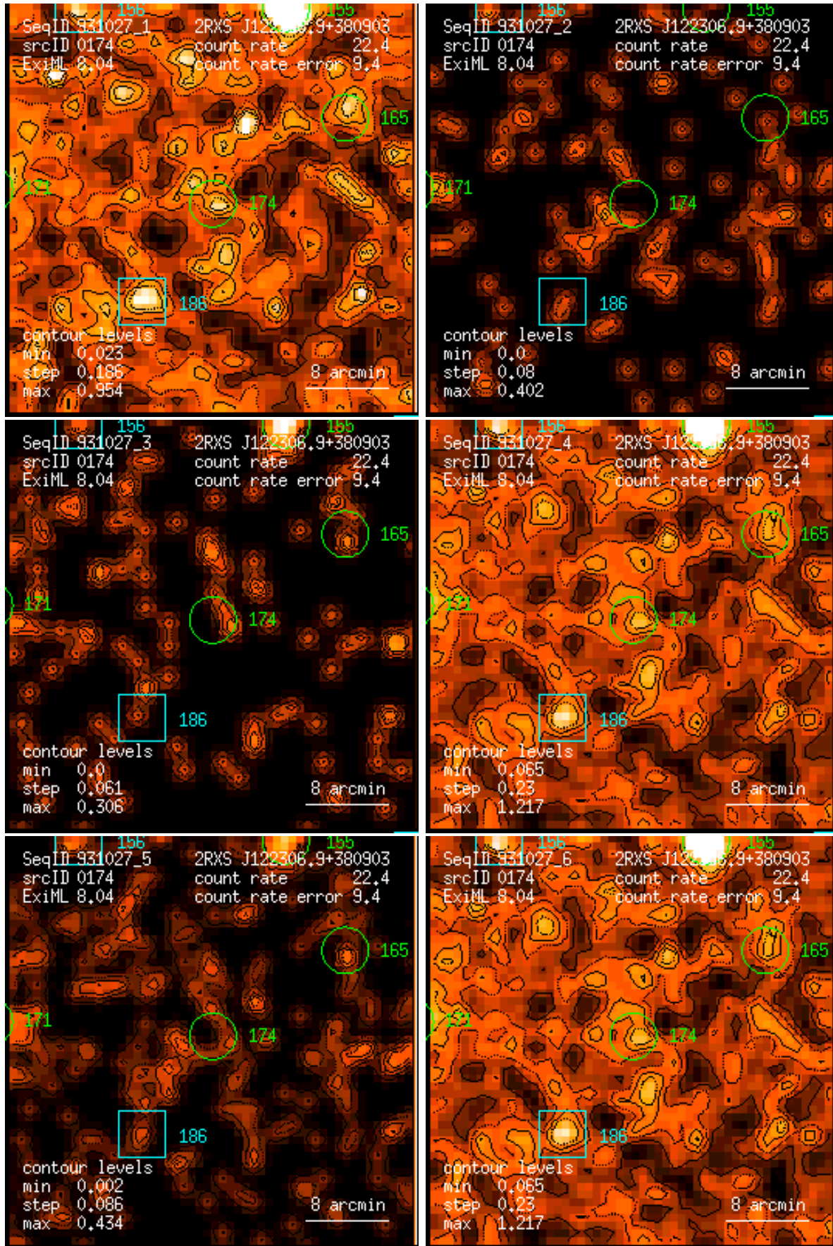
Figure 174: RASS 931027: detection 0174: band rate images, Gaussian filter: (1) PSPC channels 11 – 41, (2) 52 – 90, (3) 91 – 201, (4) 11 – 235, (5) 52 – 201, (6) 11 – 201. Broad band rates in counts/ks. Band rate contour levels in counts/ks/arcmin 2 .
