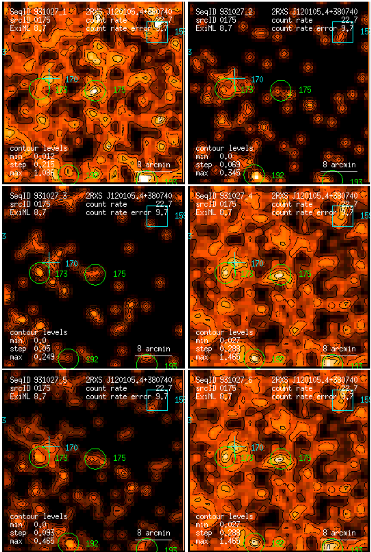
Figure 175: RASS 931027: detection 0175: band rate images, Gaussian filter: (1) PSPC channels 11 – 41, (2) 52 – 90, (3) 91 – 201, (4) 11 – 235, (5) 52 – 201, (6) 11 – 201. Broad band rates in counts/ks. Band rate contour levels in counts/ks/arcmin 2 .
