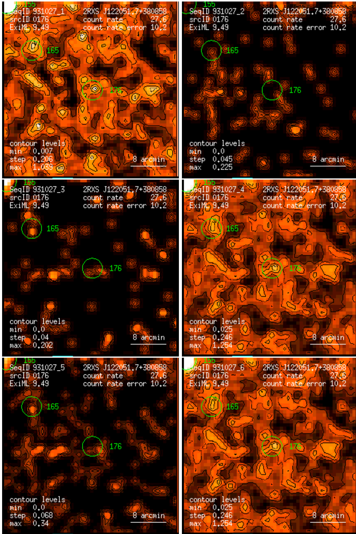
Figure 176: RASS 931027: detection 0176: band rate images, Gaussian filter: (1) PSPC channels 11 – 41, (2) 52 – 90, (3) 91 – 201, (4) 11 – 235, (5) 52 – 201, (6) 11 – 201. Broad band rates in counts/ks. Band rate contour levels in counts/ks/arcmin 2 .
