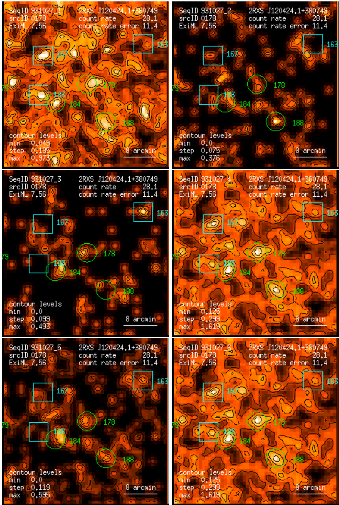
Figure 178: RASS 931027: detection 0178: band rate images, Gaussian filter: (1) PSPC channels 11 – 41, (2) 52 – 90, (3) 91 – 201, (4) 11 – 235, (5) 52 – 201, (6) 11 – 201. Broad band rates in counts/ks. Band rate contour levels in counts/ks/arcmin 2 .
