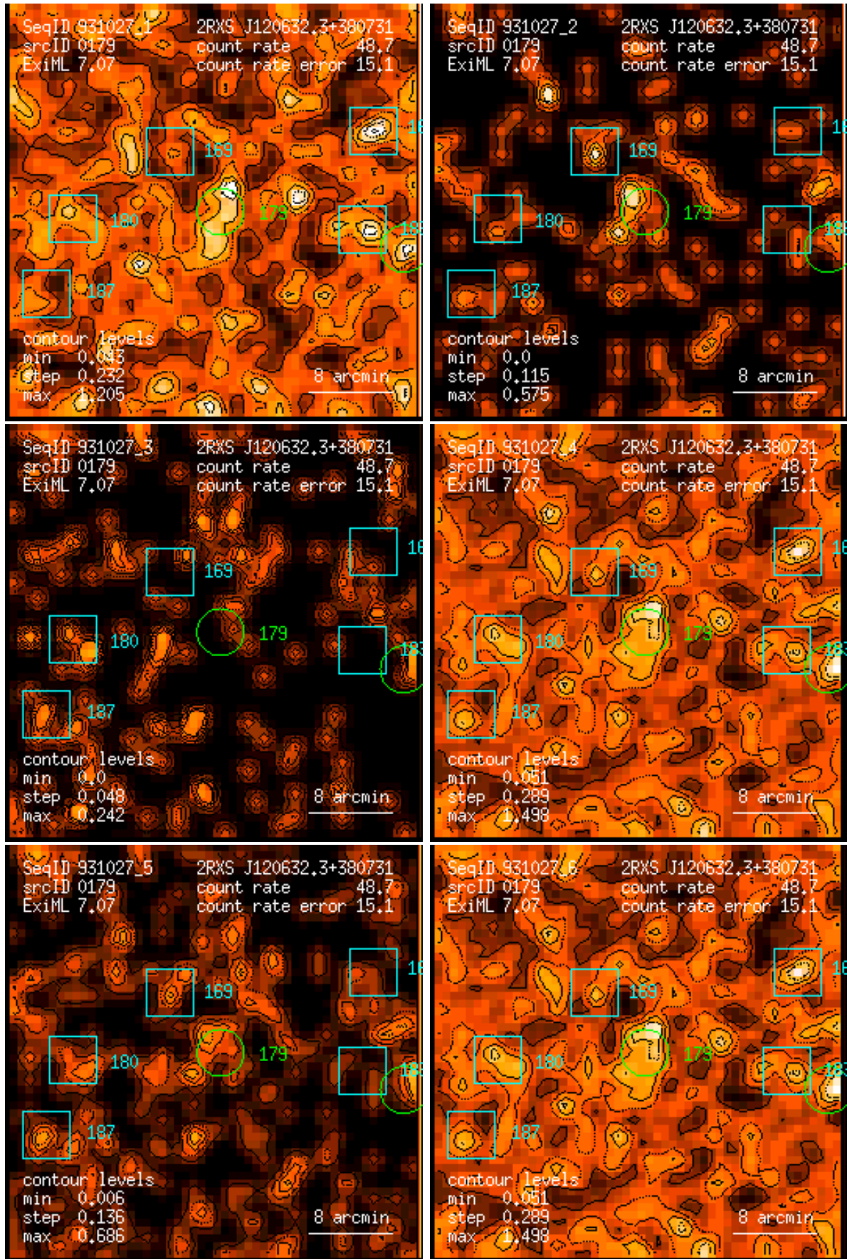
Figure 179: RASS 931027: detection 0179: band rate images, Gaussian filter: (1) PSPC channels 11 – 41, (2) 52 – 90, (3) 91 – 201, (4) 11 – 235, (5) 52 – 201, (6) 11 – 201. Broad band rates in counts/ks. Band rate contour levels in counts/ks/arcmin 2 .
