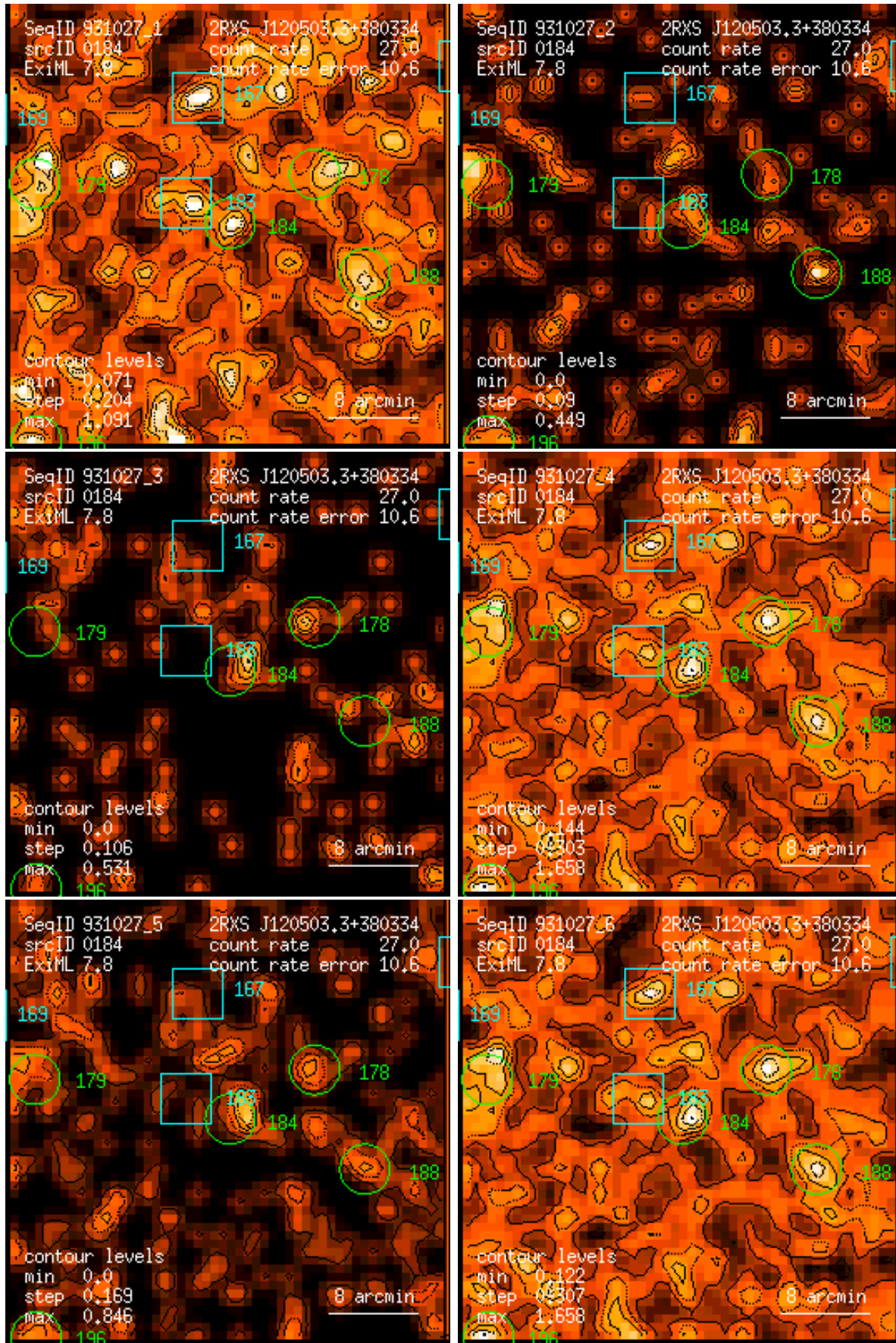
Figure 184: RASS 931027: detection 0184: band rate images, Gaussian filter: (1) PSPC channels 11 – 41, (2) 52 – 90, (3) 91 – 201, (4) 11 – 235, (5) 52 – 201, (6) 11 – 201. Broad band rates in counts/ks. Band rate contour levels in counts/ks/arcmin 2 .
