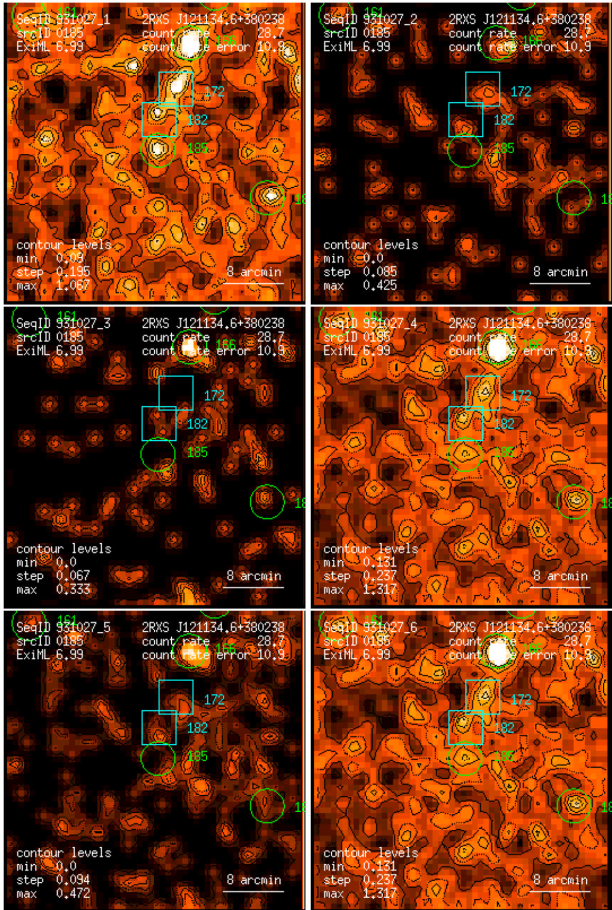
Figure 185: RASS 931027: detection 0185: band rate images, Gaussian filter: (1) PSPC channels 11 – 41, (2) 52 – 90, (3) 91 – 201, (4) 11 – 235, (5) 52 – 201, (6) 11 – 201. Broad band rates in counts/ks. Band rate contour levels in counts/ks/arcmin 2 .
