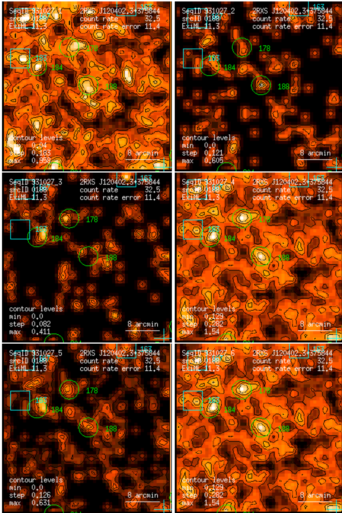
Figure 188: RASS 931027: detection 0188: band rate images, Gaussian filter: (1) PSPC channels 11 – 41, (2) 52 – 90, (3) 91 – 201, (4) 11 – 235, (5) 52 – 201, (6) 11 – 201. Broad band rates in counts/ks. Band rate contour levels in counts/ks/arcmin 2 .
