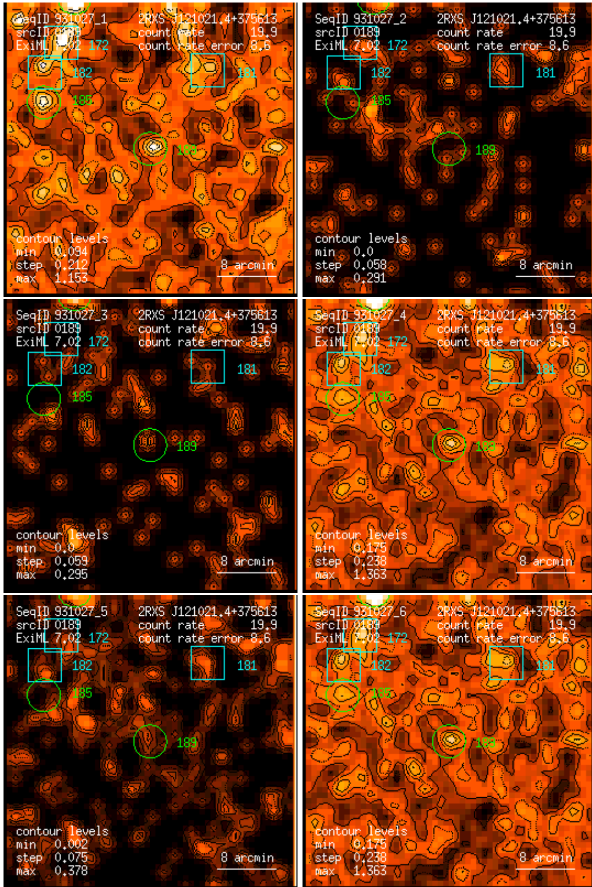
Figure 189: RASS 931027: detection 0189: band rate images, Gaussian filter: (1) PSPC channels 11 – 41, (2) 52 – 90, (3) 91 – 201, (4) 11 – 235, (5) 52 – 201, (6) 11 – 201. Broad band rates in counts/ks. Band rate contour levels in counts/ks/arcmin 2 .
