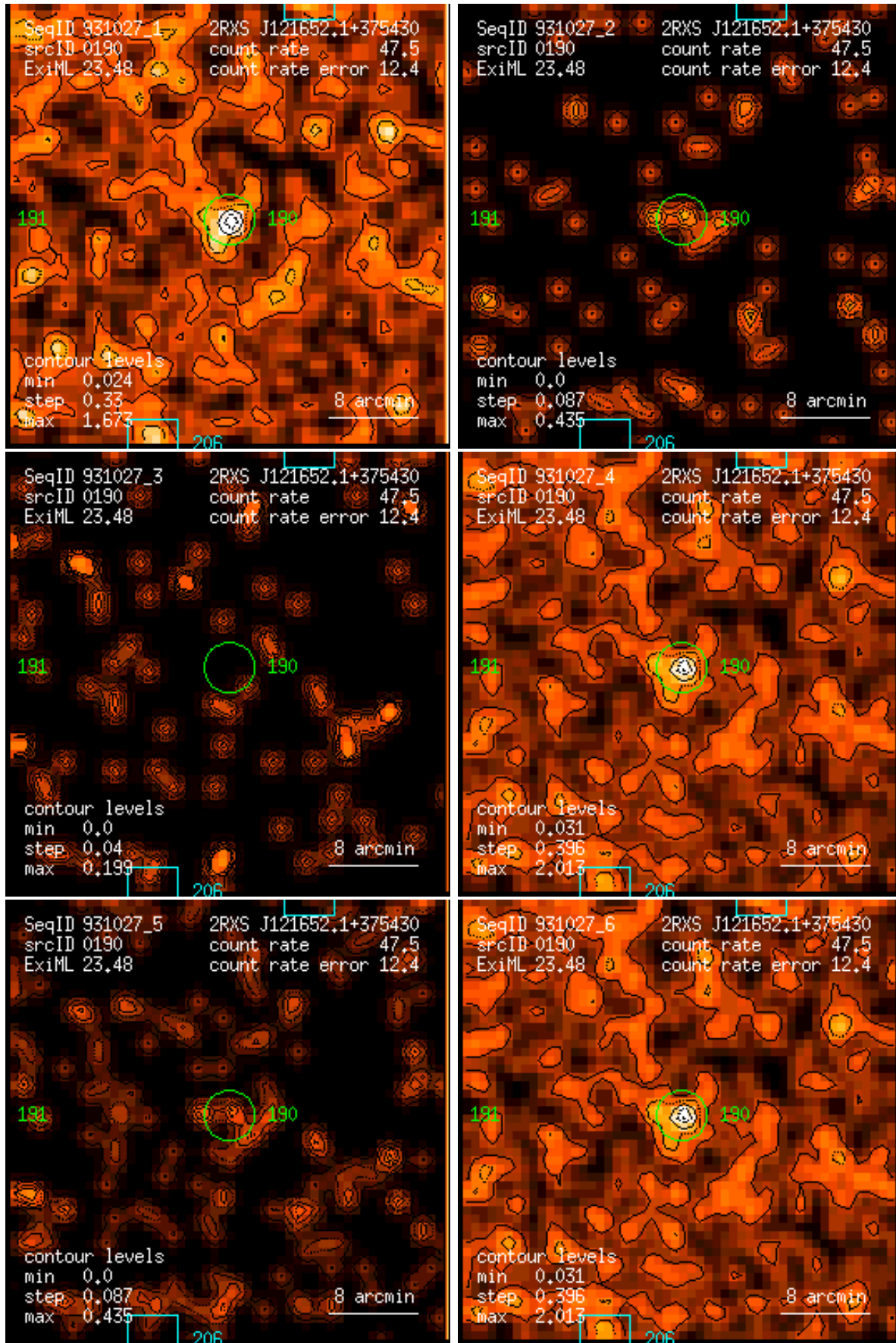
Figure 190: RASS 931027: detection 0190: band rate images, Gaussian filter: (1) PSPC channels 11 – 41, (2) 52 – 90, (3) 91 – 201, (4) 11 – 235, (5) 52 – 201, (6) 11 – 201. Broad band rates in counts/ks. Band rate contour levels in counts/ks/arcmin 2 .
