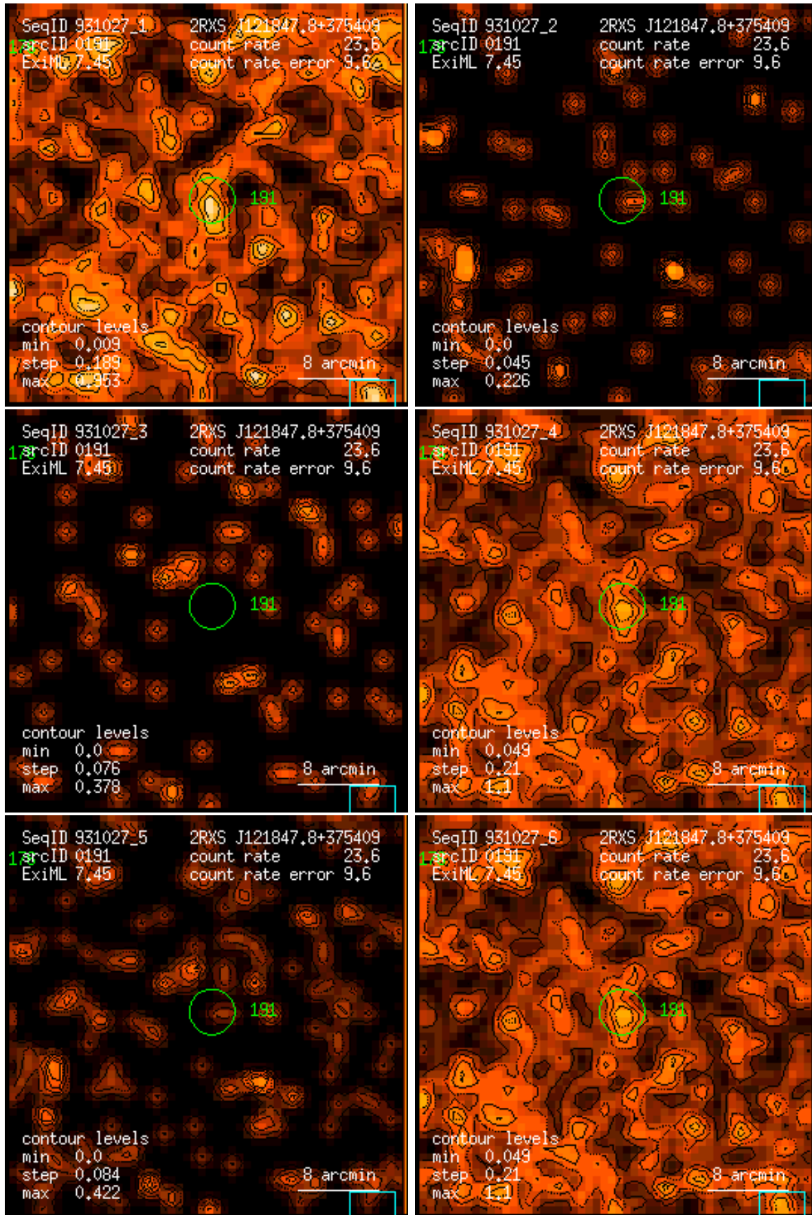
Figure 191: RASS 931027: detection 0191: band rate images, Gaussian filter: (1) PSPC channels 11 – 41, (2) 52 – 90, (3) 91 – 201, (4) 11 – 235, (5) 52 – 201, (6) 11 – 201. Broad band rates in counts/ks. Band rate contour levels in counts/ks/arcmin 2 .
