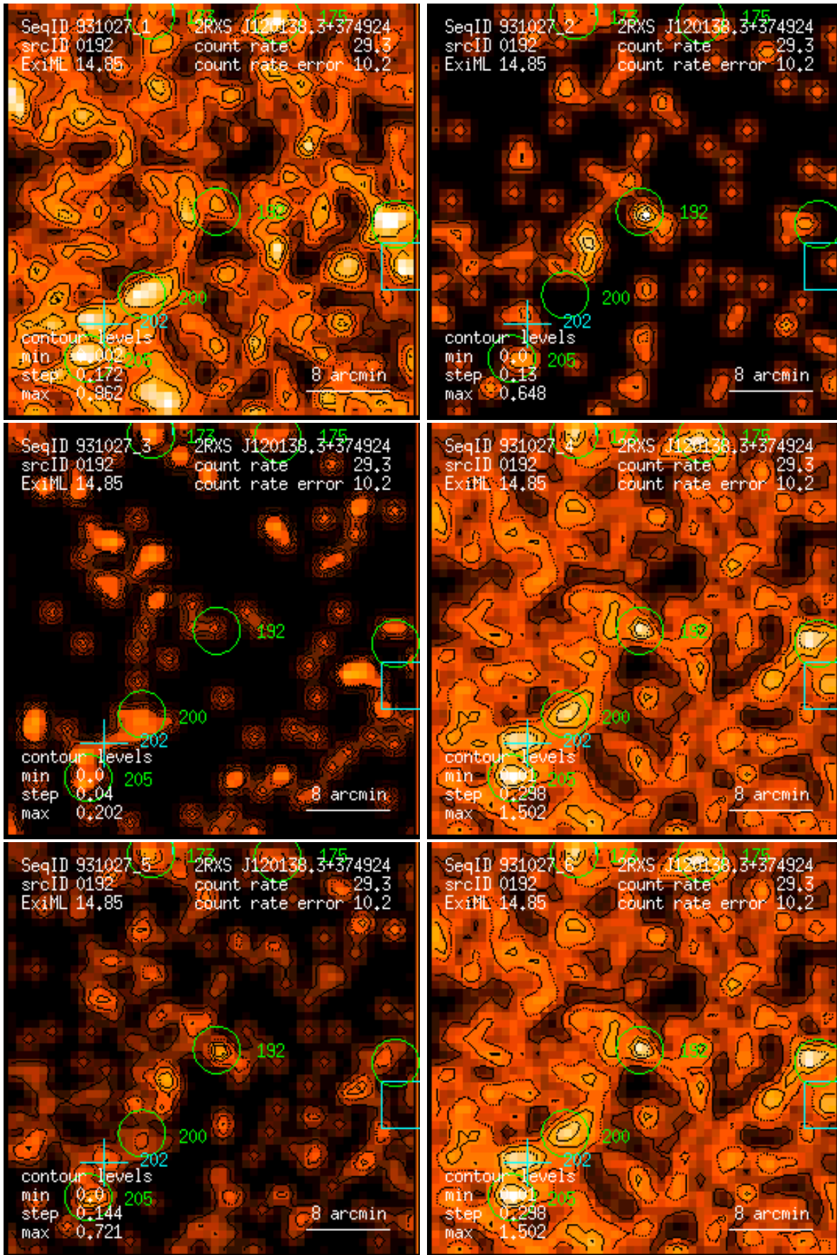
Figure 192: RASS 931027: detection 0192: band rate images, Gaussian filter: (1) PSPC channels 11 – 41, (2) 52 – 90, (3) 91 – 201, (4) 11 – 235, (5) 52 – 201, (6) 11 – 201. Broad band rates in counts/ks. Band rate contour levels in counts/ks/arcmin 2 .
