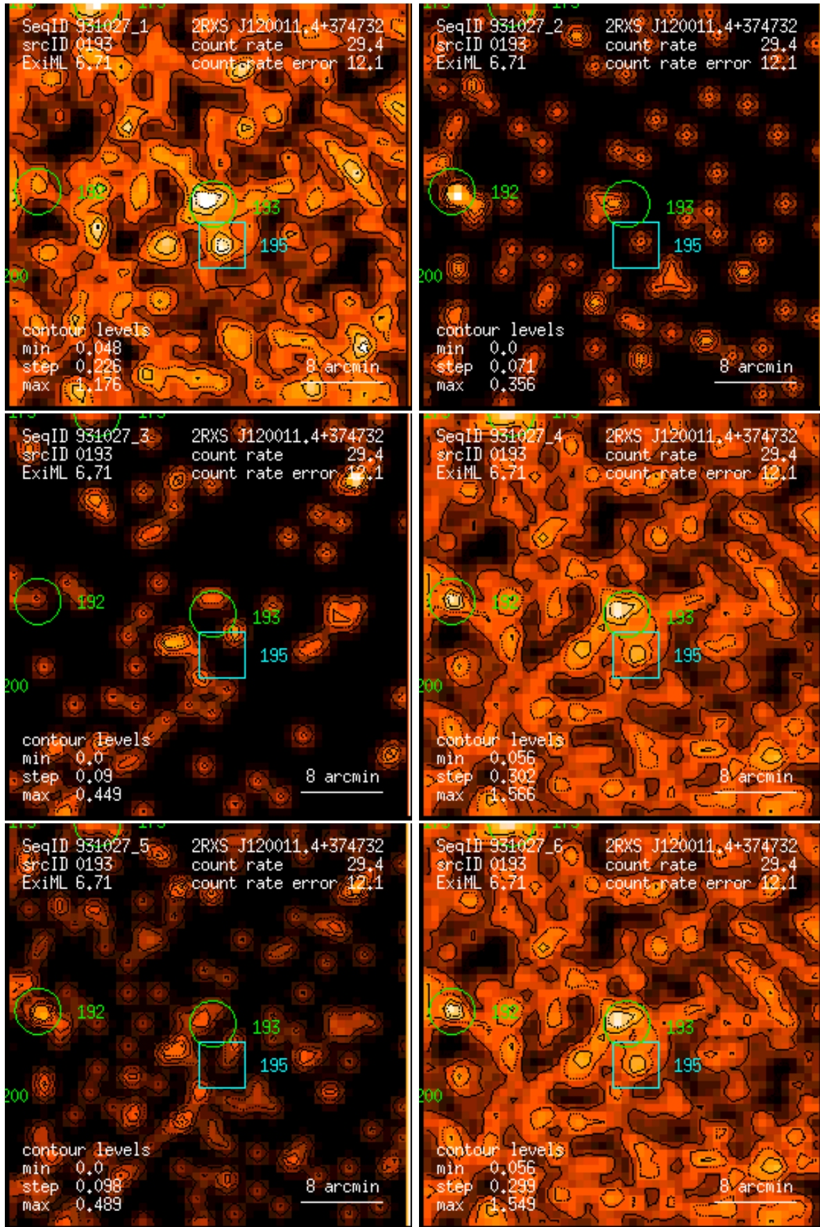
Figure 193: RASS 931027: detection 0193: band rate images, Gaussian filter: (1) PSPC channels 11 – 41, (2) 52 – 90, (3) 91 – 201, (4) 11 – 235, (5) 52 – 201, (6) 11 – 201. Broad band rates in counts/ks. Band rate contour levels in counts/ks/arcmin 2 .
