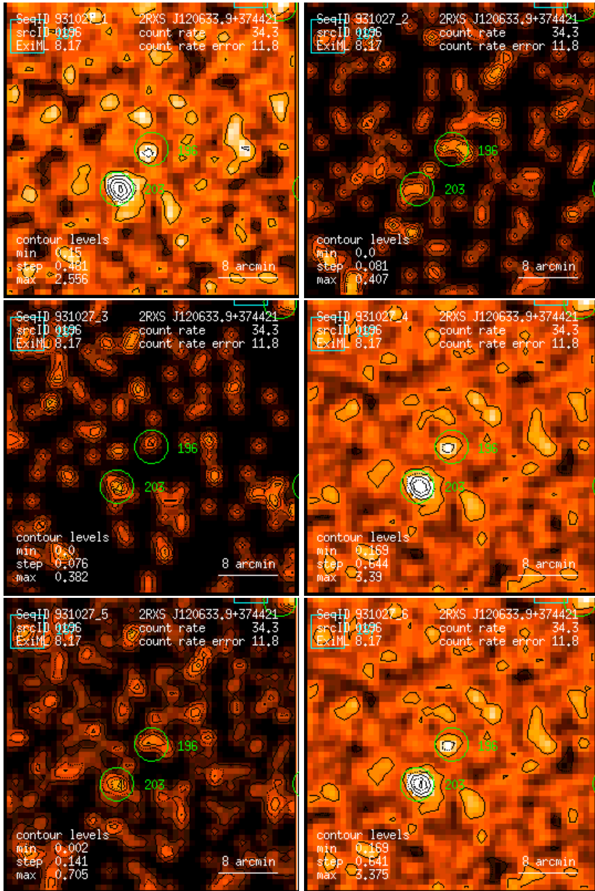
Figure 196: RASS 931027: detection 0196: band rate images, Gaussian filter: (1) PSPC channels 11 – 41, (2) 52 – 90, (3) 91 – 201, (4) 11 – 235, (5) 52 – 201, (6) 11 – 201. Broad band rates in counts/ks. Band rate contour levels in counts/ks/arcmin 2 .
