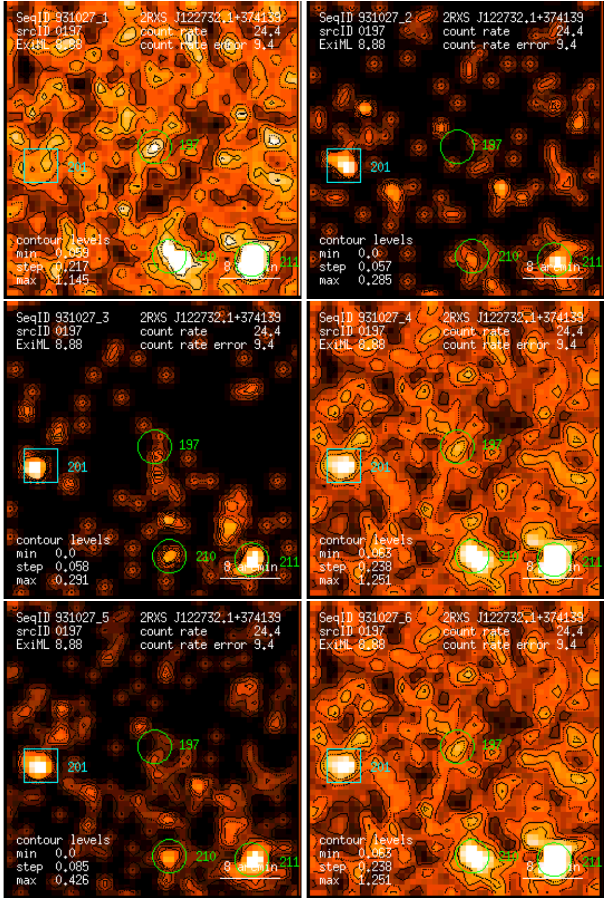
Figure 197: RASS 931027: detection 0197: band rate images, Gaussian filter: (1) PSPC channels 11 – 41, (2) 52 – 90, (3) 91 – 201, (4) 11 – 235, (5) 52 – 201, (6) 11 – 201. Broad band rates in counts/ks. Band rate contour levels in counts/ks/arcmin 2 .
