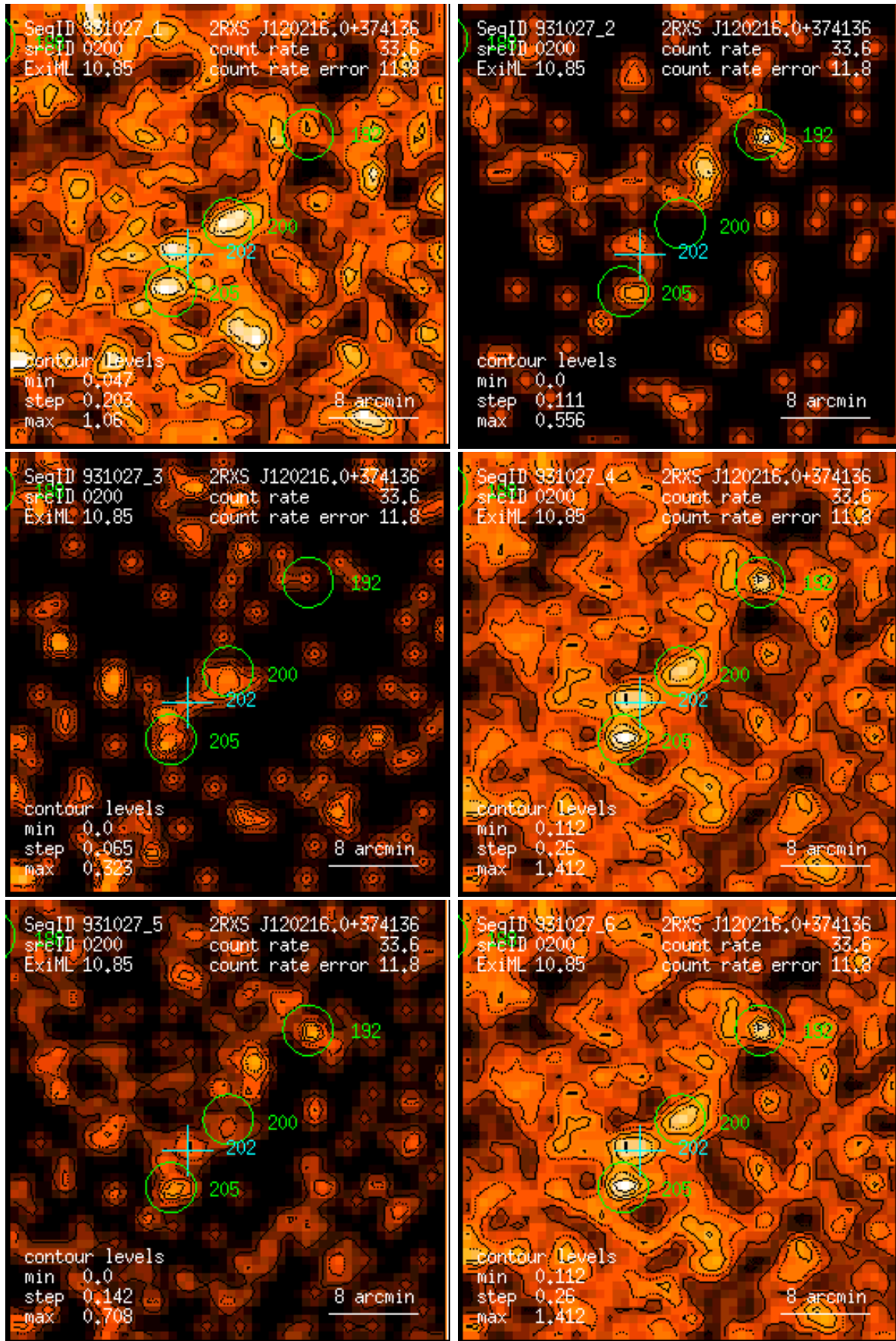
Figure 200: RASS 931027: detection 0200: band rate images, Gaussian filter: (1) PSPC channels 11 – 41, (2) 52 – 90, (3) 91 – 201, (4) 11 – 235, (5) 52 – 201, (6) 11 – 201. Broad band rates in counts/ks. Band rate contour levels in counts/ks/arcmin 2 .
