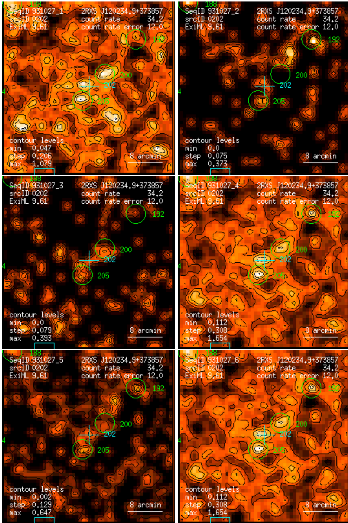
Figure 202: RASS 931027: detection 0202: band rate images, Gaussian filter: (1) PSPC channels 11 – 41, (2) 52 – 90, (3) 91 – 201, (4) 11 – 235, (5) 52 – 201, (6) 11 – 201. Broad band rates in counts/ks. Band rate contour levels in counts/ks/arcmin 2 .
