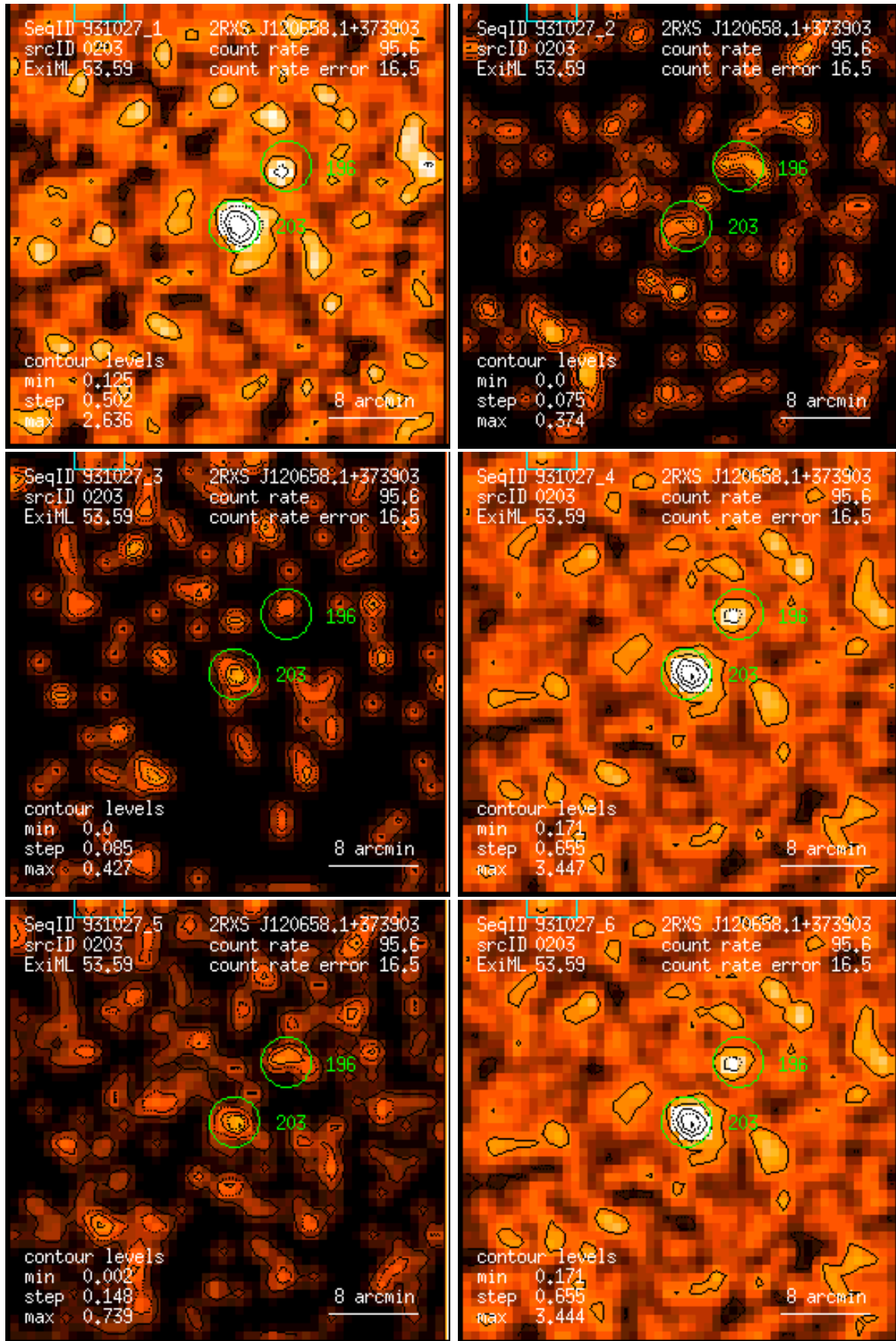
Figure 203: RASS 931027: detection 0203: band rate images, Gaussian filter: (1) PSPC channels 11 – 41, (2) 52 – 90, (3) 91 – 201, (4) 11 – 235, (5) 52 – 201, (6) 11 – 201. Broad band rates in counts/ks. Band rate contour levels in counts/ks/arcmin 2 .
