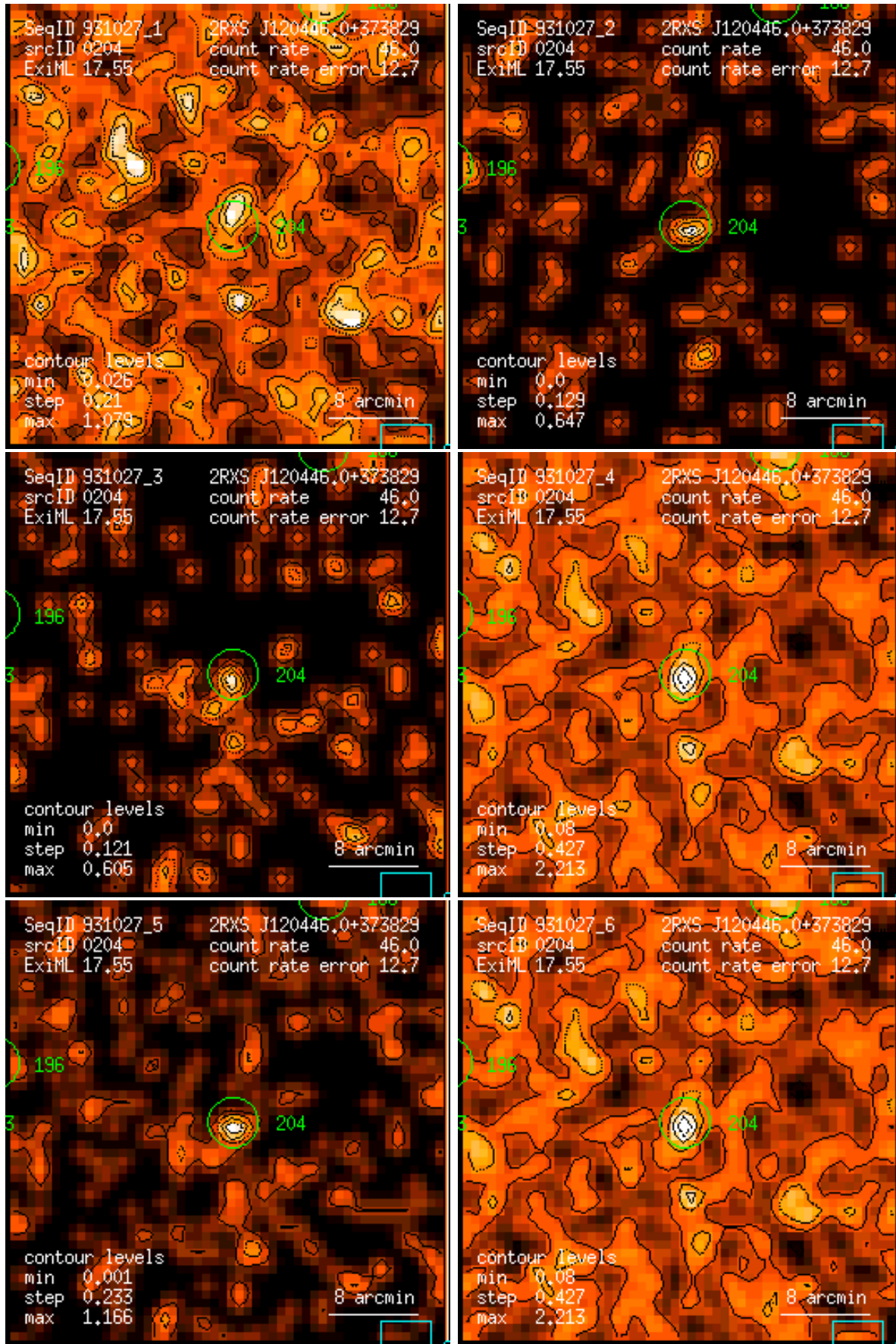
Figure 204: RASS 931027: detection 0204: band rate images, Gaussian filter: (1) PSPC channels 11 – 41, (2) 52 – 90, (3) 91 – 201, (4) 11 – 235, (5) 52 – 201, (6) 11 – 201. Broad band rates in counts/ks. Band rate contour levels in counts/ks/arcmin 2 .
