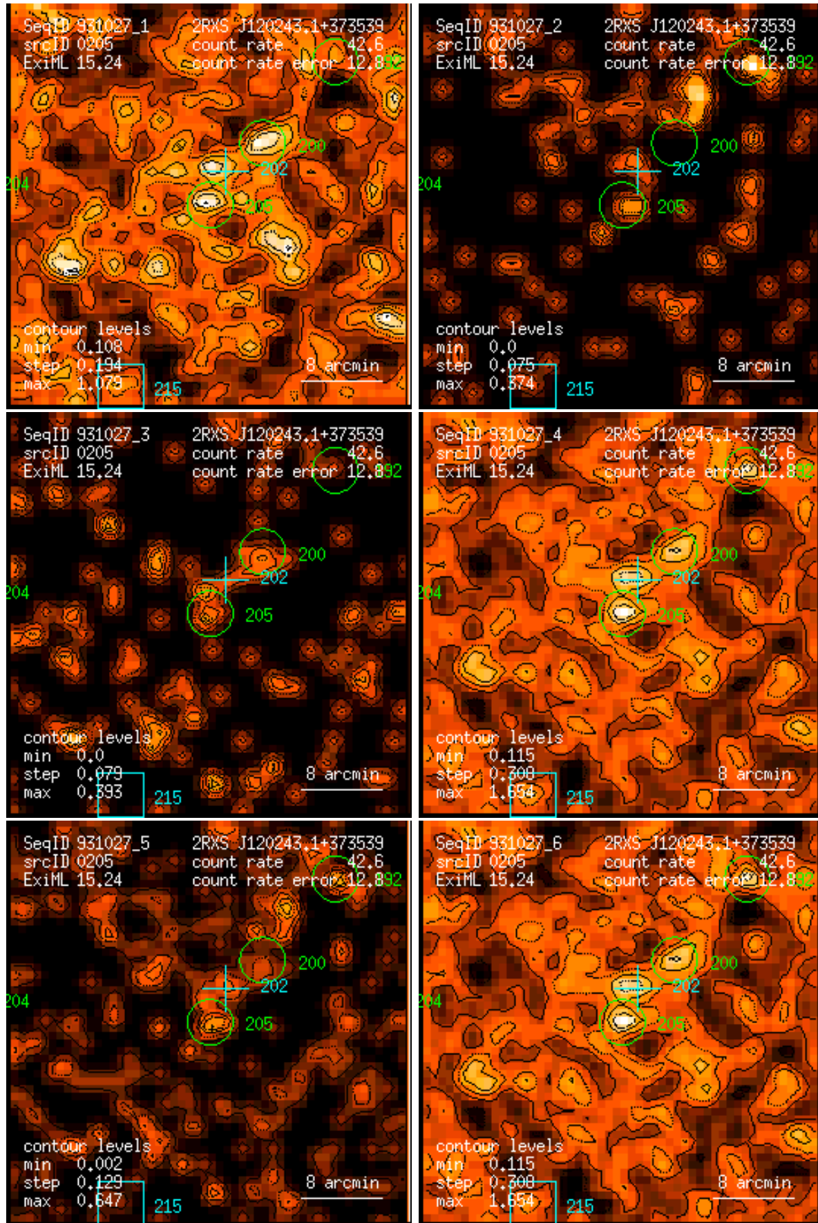
Figure 205: RASS 931027: detection 0205: band rate images, Gaussian filter: (1) PSPC channels 11 – 41, (2) 52 – 90, (3) 91 – 201, (4) 11 – 235, (5) 52 – 201, (6) 11 – 201. Broad band rates in counts/ks. Band rate contour levels in counts/ks/arcmin 2 .
