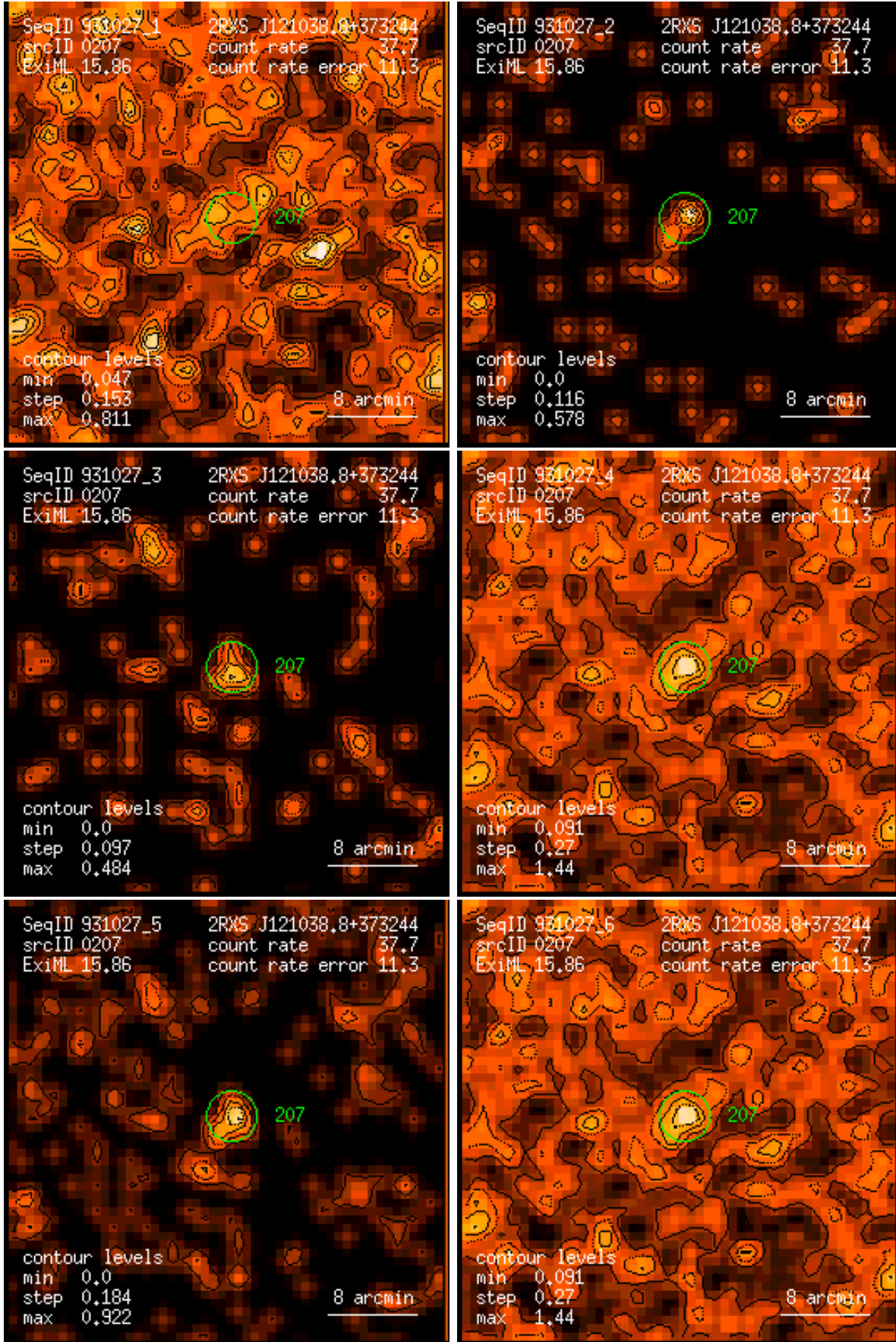
Figure 207: RASS 931027: detection 0207: band rate images, Gaussian filter: (1) PSPC channels 11 – 41, (2) 52 – 90, (3) 91 – 201, (4) 11 – 235, (5) 52 – 201, (6) 11 – 201. Broad band rates in counts/ks. Band rate contour levels in counts/ks/arcmin 2 .
