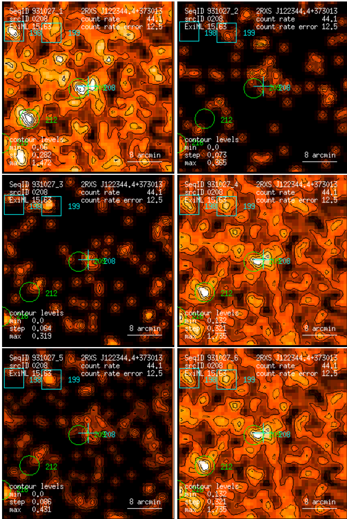
Figure 208: RASS 931027: detection 0208: band rate images, Gaussian filter: (1) PSPC channels 11 – 41, (2) 52 – 90, (3) 91 – 201, (4) 11 – 235, (5) 52 – 201, (6) 11 – 201. Broad band rates in counts/ks. Band rate contour levels in counts/ks/arcmin 2 .
