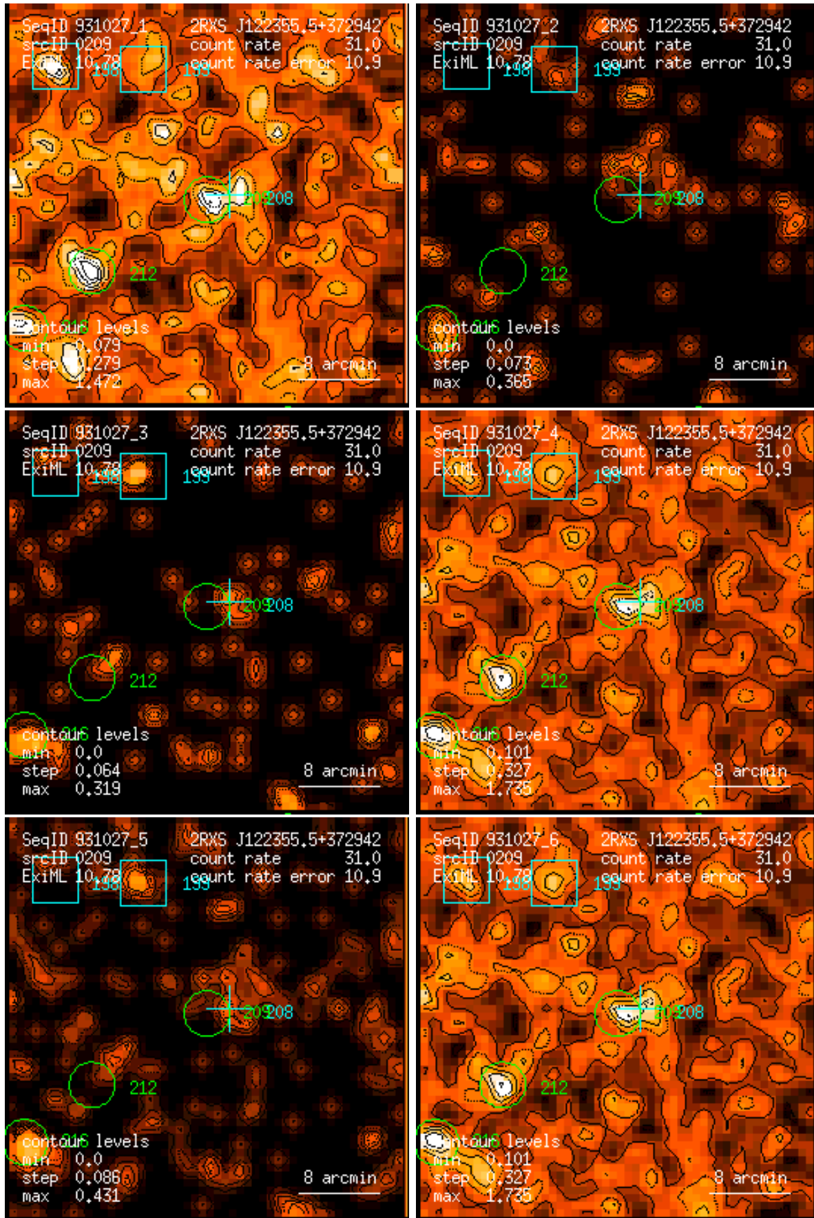
Figure 209: RASS 931027: detection 0209: band rate images, Gaussian filter: (1) PSPC channels 11 – 41, (2) 52 – 90, (3) 91 – 201, (4) 11 – 235, (5) 52 – 201, (6) 11 – 201. Broad band rates in counts/ks. Band rate contour levels in counts/ks/arcmin 2 .
