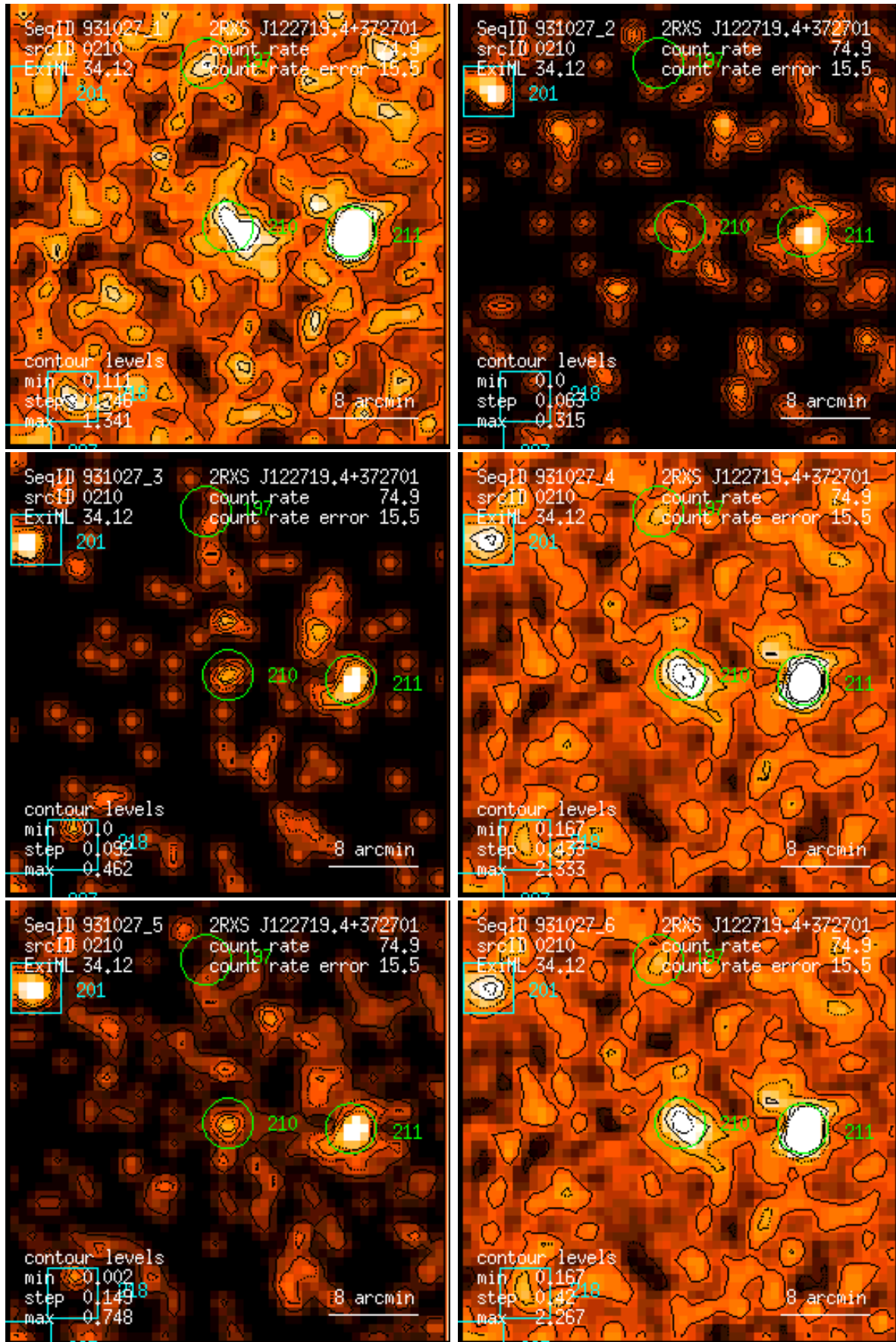
Figure 210: RASS 931027: detection 0210: band rate images, Gaussian filter: (1) PSPC channels 11 – 41, (2) 52 – 90, (3) 91 – 201, (4) 11 – 235, (5) 52 – 201, (6) 11 – 201. Broad band rates in counts/ks. Band rate contour levels in counts/ks/arcmin 2 .
