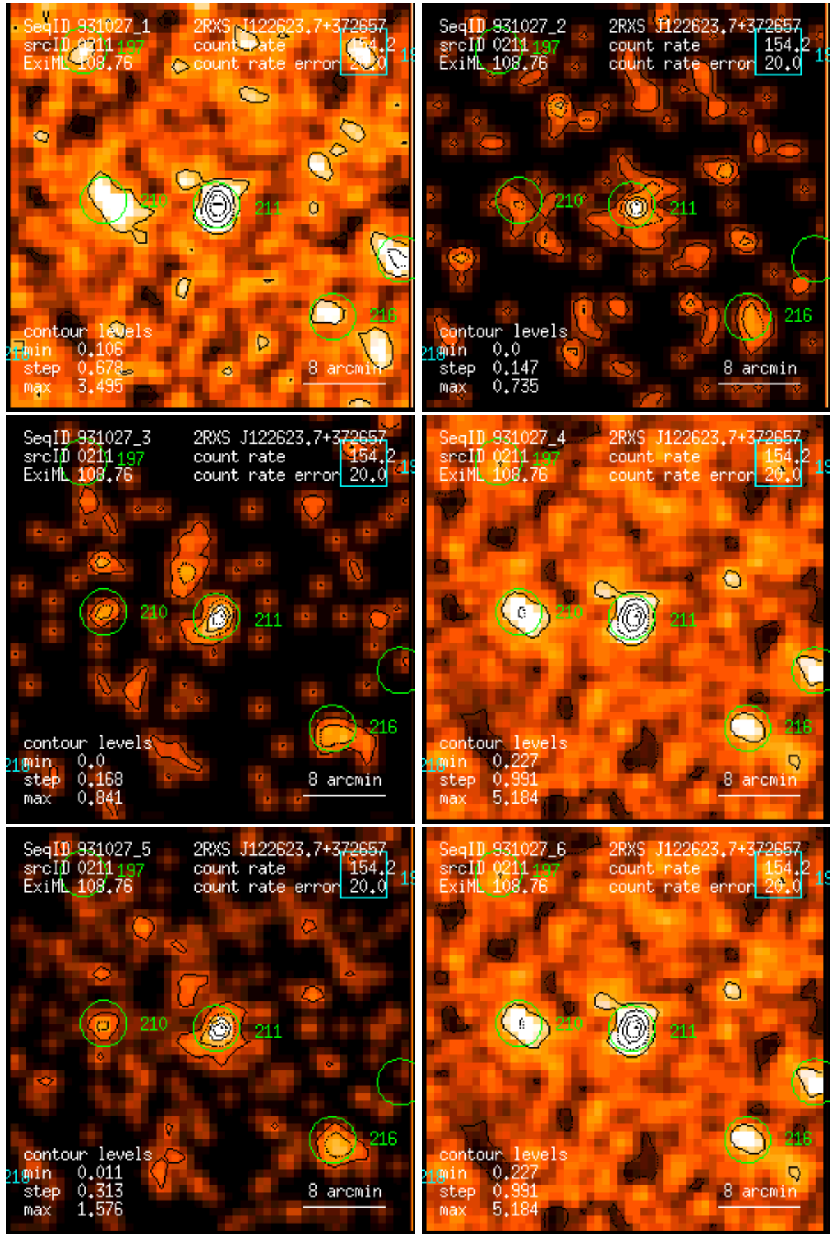
Figure 211: RASS 931027: detection 0211: band rate images, Gaussian filter: (1) PSPC channels 11 – 41, (2) 52 – 90, (3) 91 – 201, (4) 11 – 235, (5) 52 – 201, (6) 11 – 201. Broad band rates in counts/ks. Band rate contour levels in counts/ks/arcmin 2 .
