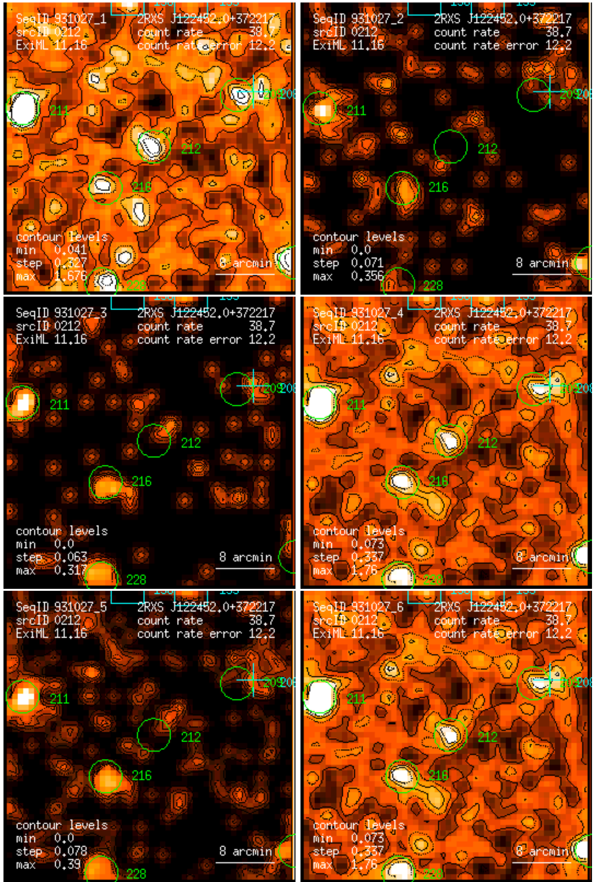
Figure 212: RASS 931027: detection 0212: band rate images, Gaussian filter: (1) PSPC channels 11 – 41, (2) 52 – 90, (3) 91 – 201, (4) 11 – 235, (5) 52 – 201, (6) 11 – 201. Broad band rates in counts/ks. Band rate contour levels in counts/ks/arcmin 2 .
