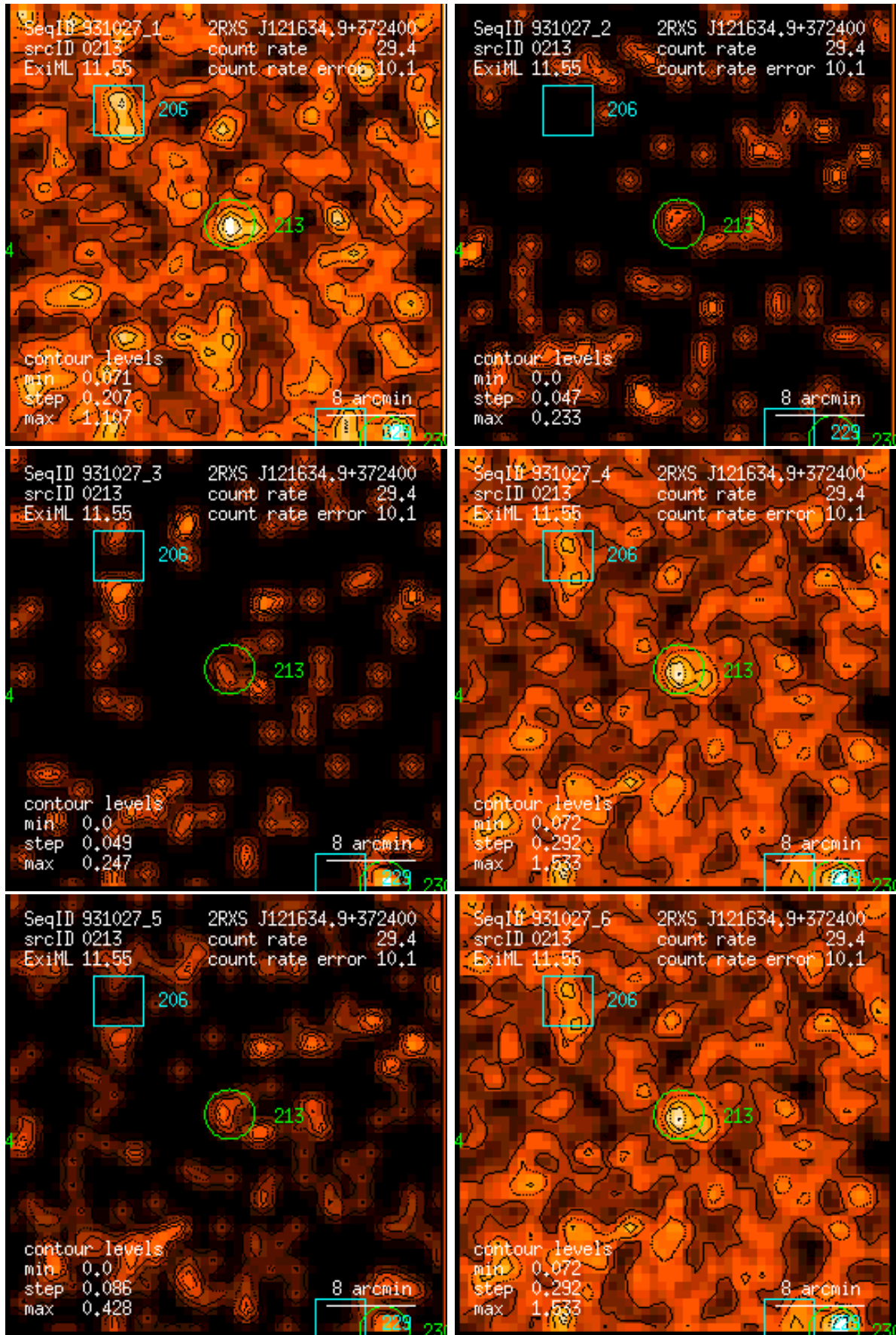
Figure 213: RASS 931027: detection 0213: band rate images, Gaussian filter: (1) PSPC channels 11 – 41, (2) 52 – 90, (3) 91 – 201, (4) 11 – 235, (5) 52 – 201, (6) 11 – 201. Broad band rates in counts/ks. Band rate contour levels in counts/ks/arcmin 2 .
