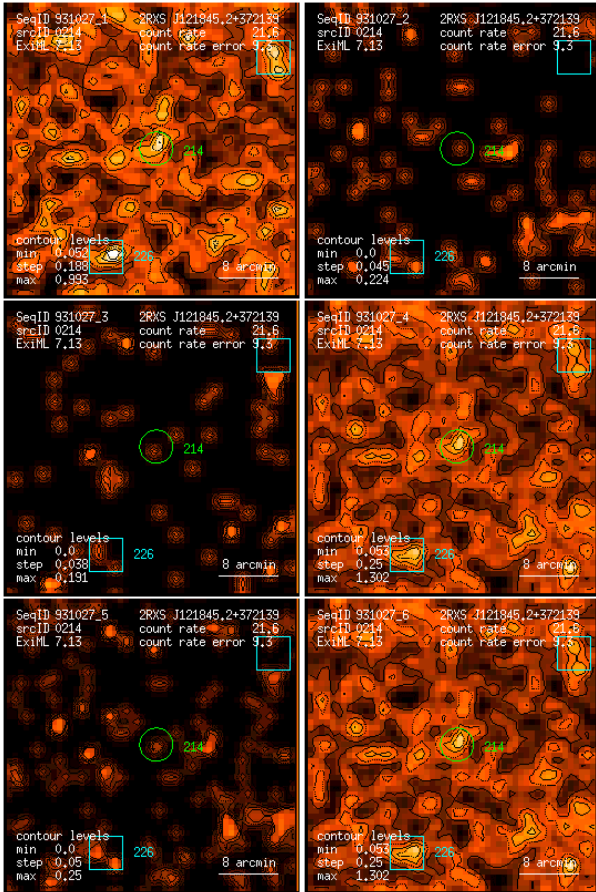
Figure 214: RASS 931027: detection 0214: band rate images, Gaussian filter: (1) PSPC channels 11 – 41, (2) 52 – 90, (3) 91 – 201, (4) 11 – 235, (5) 52 – 201, (6) 11 – 201. Broad band rates in counts/ks. Band rate contour levels in counts/ks/arcmin 2 .
