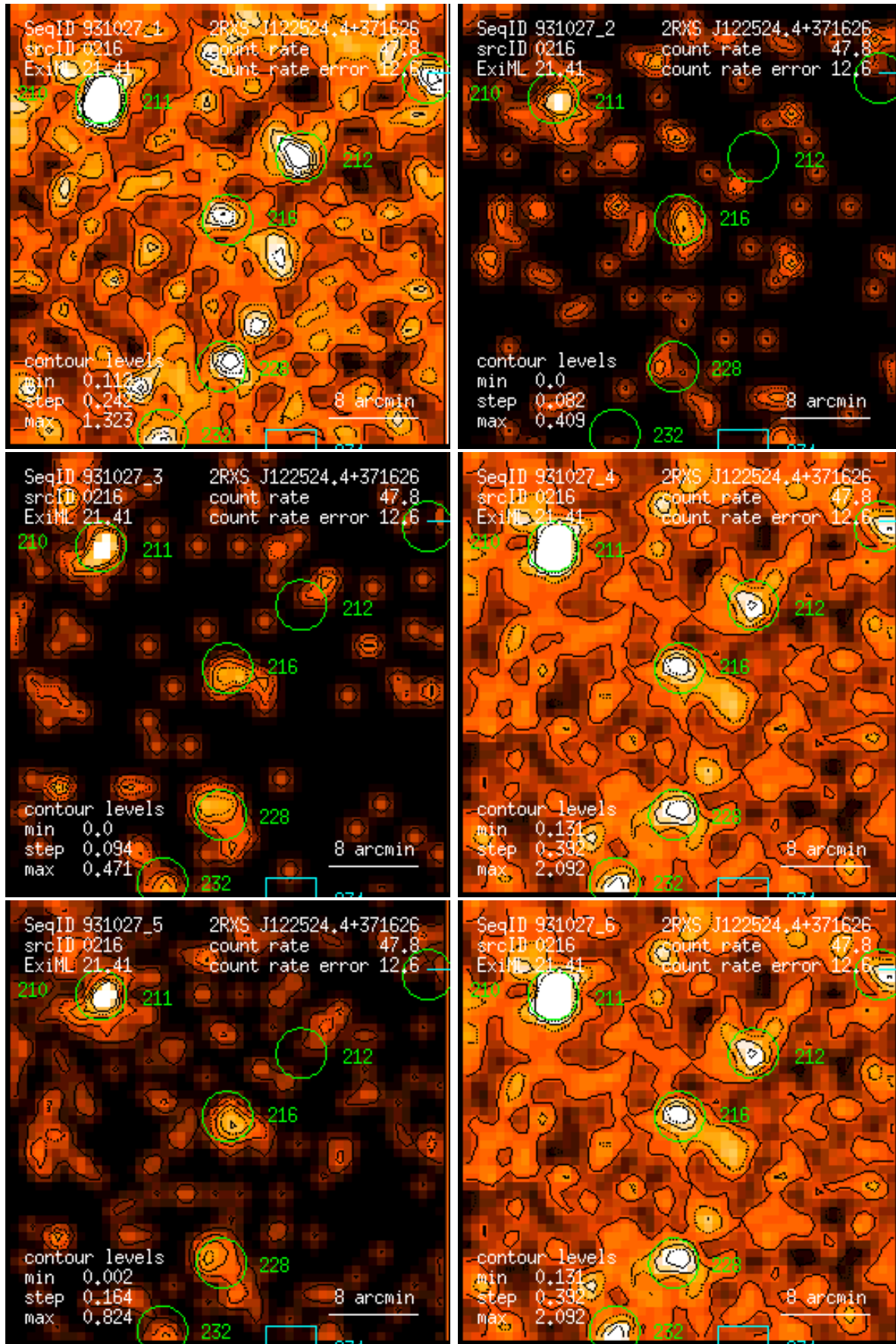
Figure 216: RASS 931027: detection 0216: band rate images, Gaussian filter: (1) PSPC channels 11 – 41, (2) 52 – 90, (3) 91 – 201, (4) 11 – 235, (5) 52 – 201, (6) 11 – 201. Broad band rates in counts/ks. Band rate contour levels in counts/ks/arcmin 2 .
