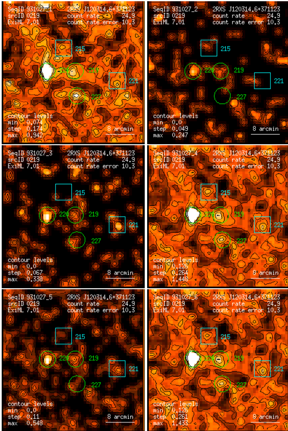
Figure 219: RASS 931027: detection 0219: band rate images, Gaussian filter: (1) PSPC channels 11 – 41, (2) 52 – 90, (3) 91 – 201, (4) 11 – 235, (5) 52 – 201, (6) 11 – 201. Broad band rates in counts/ks. Band rate contour levels in counts/ks/arcmin 2 .
