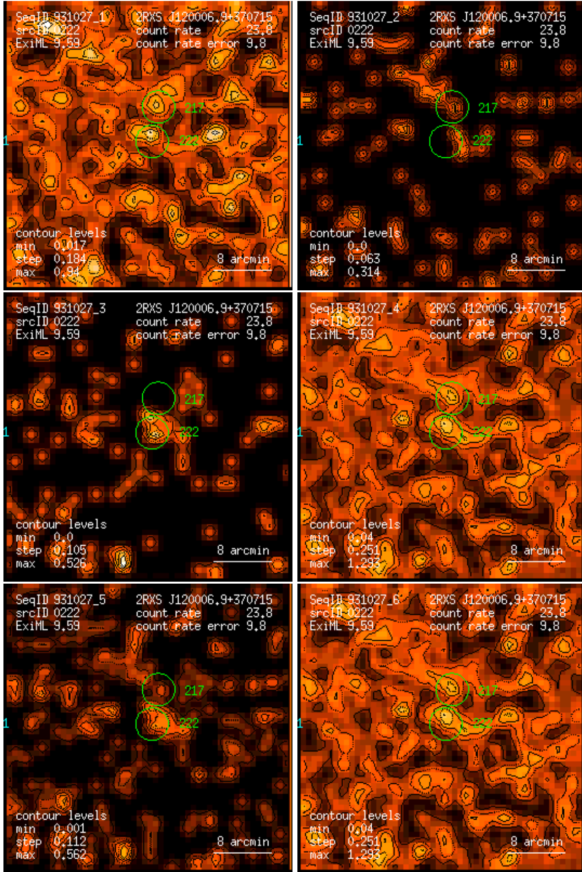
Figure 222: RASS 931027: detection 0222: band rate images, Gaussian filter: (1) PSPC channels 11 – 41, (2) 52 – 90, (3) 91 – 201, (4) 11 – 235, (5) 52 – 201, (6) 11 – 201. Broad band rates in counts/ks. Band rate contour levels in counts/ks/arcmin 2 .
