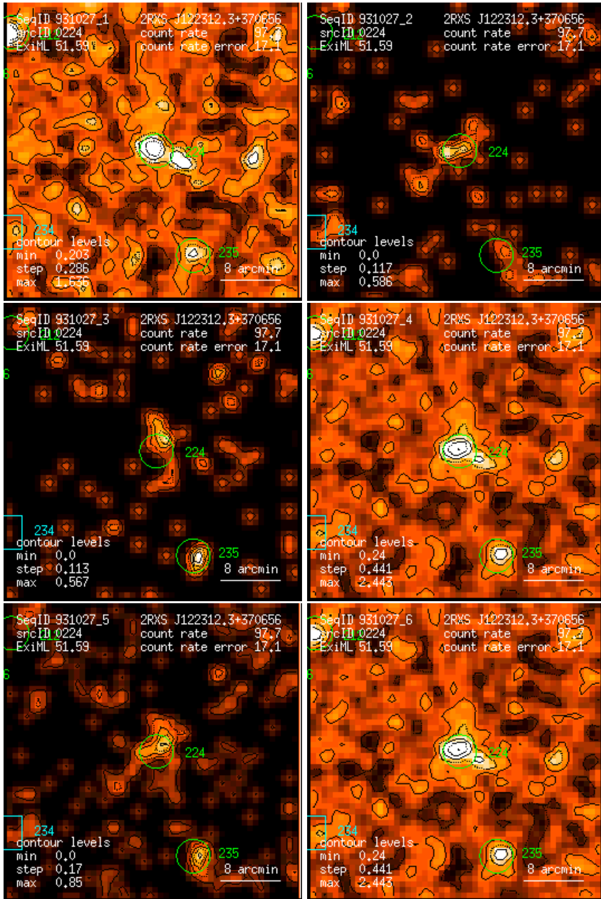
Figure 224: RASS 931027: detection 0224: band rate images, Gaussian filter: (1) PSPC channels 11 – 41, (2) 52 – 90, (3) 91 – 201, (4) 11 – 235, (5) 52 – 201, (6) 11 – 201. Broad band rates in counts/ks. Band rate contour levels in counts/ks/arcmin 2 .
