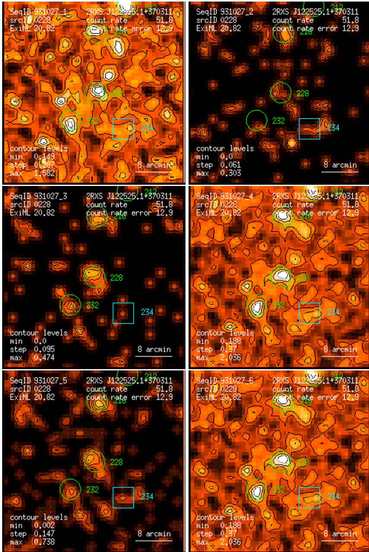
Figure 228: RASS 931027: detection 0228: band rate images, Gaussian filter: (1) PSPC channels 11 – 41, (2) 52 – 90, (3) 91 – 201, (4) 11 – 235, (5) 52 – 201, (6) 11 – 201. Broad band rates in counts/ks. Band rate contour levels in counts/ks/arcmin 2 .
