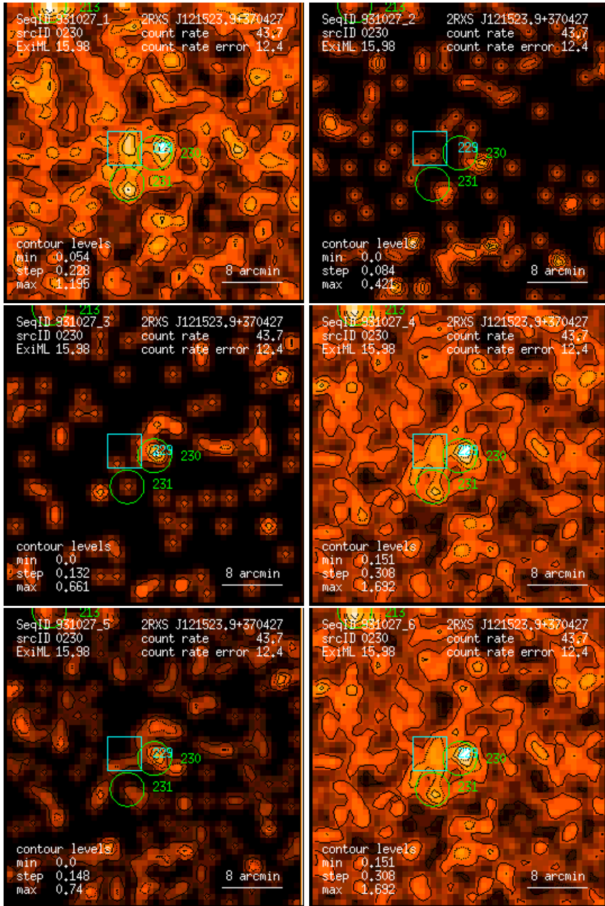
Figure 230: RASS 931027: detection 0230: band rate images, Gaussian filter: (1) PSPC channels 11 – 41, (2) 52 – 90, (3) 91 – 201, (4) 11 – 235, (5) 52 – 201, (6) 11 – 201. Broad band rates in counts/ks. Band rate contour levels in counts/ks/arcmin 2 .
