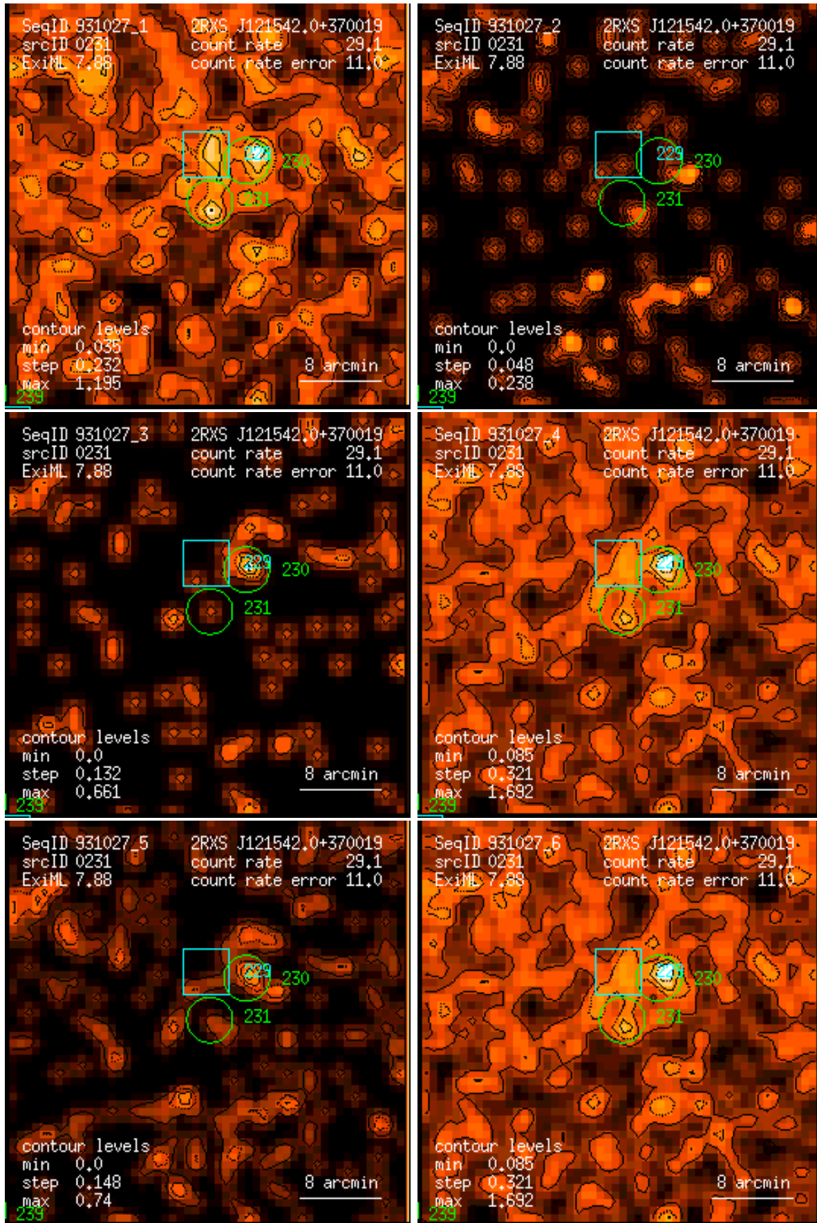
Figure 231: RASS 931027: detection 0231: band rate images, Gaussian filter: (1) PSPC channels 11 – 41, (2) 52 – 90, (3) 91 – 201, (4) 11 – 235, (5) 52 – 201, (6) 11 – 201. Broad band rates in counts/ks. Band rate contour levels in counts/ks/arcmin 2 .
