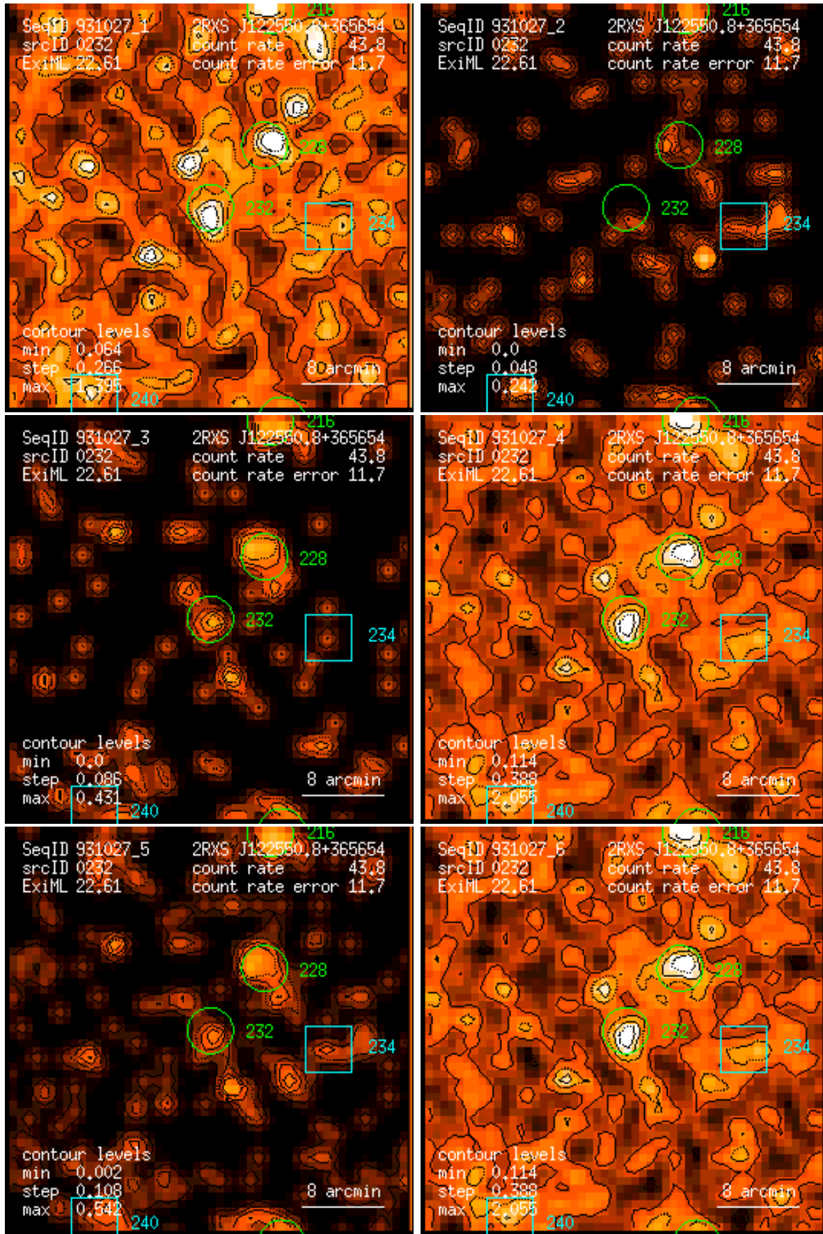
Figure 232: RASS 931027: detection 0232: band rate images, Gaussian filter: (1) PSPC channels 11 – 41, (2) 52 – 90, (3) 91 – 201, (4) 11 – 235, (5) 52 – 201, (6) 11 – 201. Broad band rates in counts/ks. Band rate contour levels in counts/ks/arcmin 2 .
