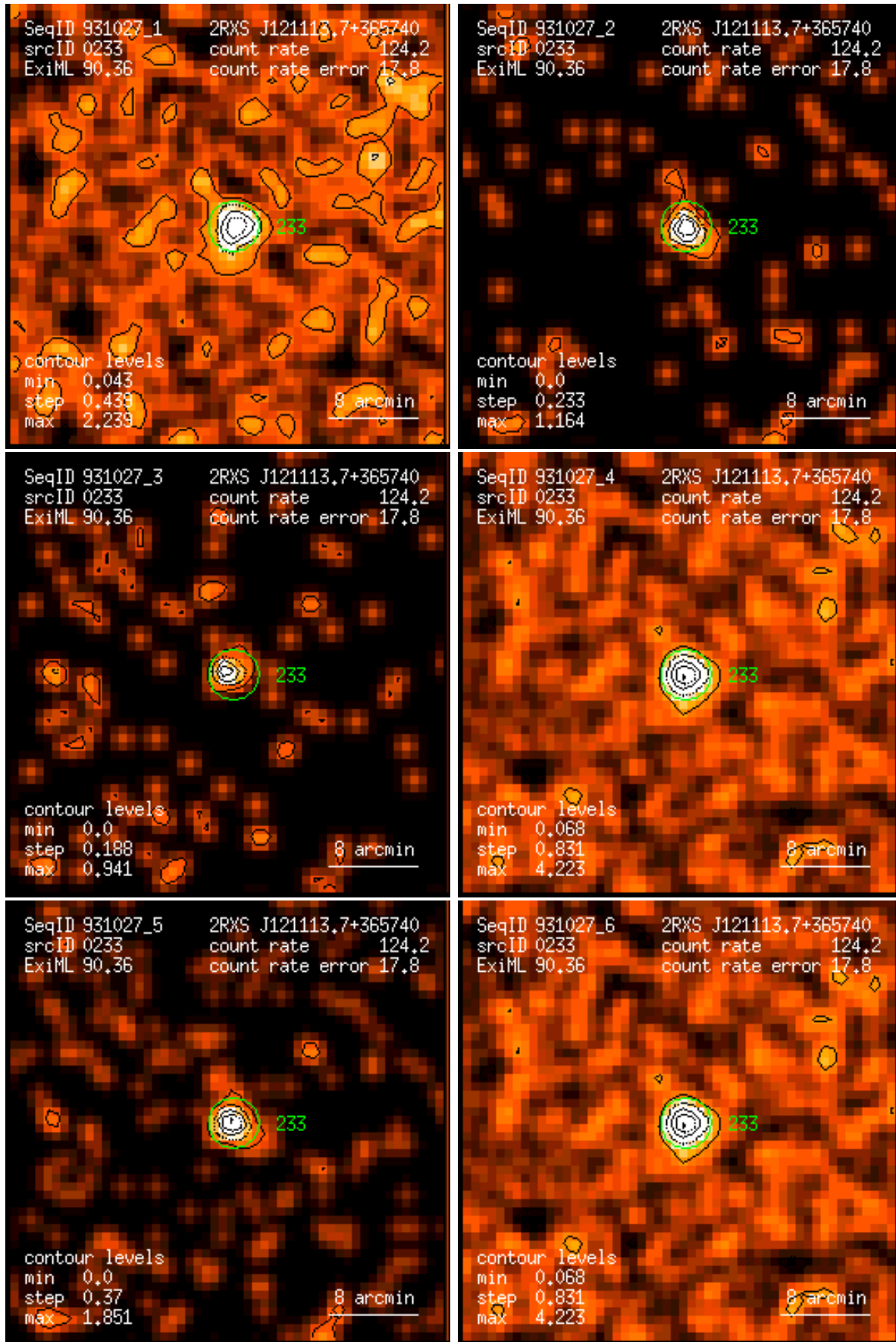
Figure 233: RASS 931027: detection 0233: band rate images, Gaussian filter: (1) PSPC channels 11 – 41, (2) 52 – 90, (3) 91 – 201, (4) 11 – 235, (5) 52 – 201, (6) 11 – 201. Broad band rates in counts/ks. Band rate contour levels in counts/ks/arcmin 2 .
