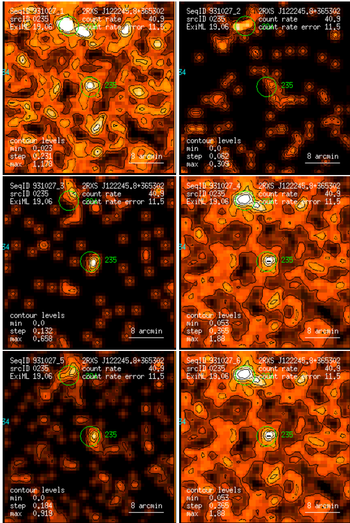
Figure 235: RASS 931027: detection 0235: band rate images, Gaussian filter: (1) PSPC channels 11 – 41, (2) 52 – 90, (3) 91 – 201, (4) 11 – 235, (5) 52 – 201, (6) 11 – 201. Broad band rates in counts/ks. Band rate contour levels in counts/ks/arcmin 2 .
