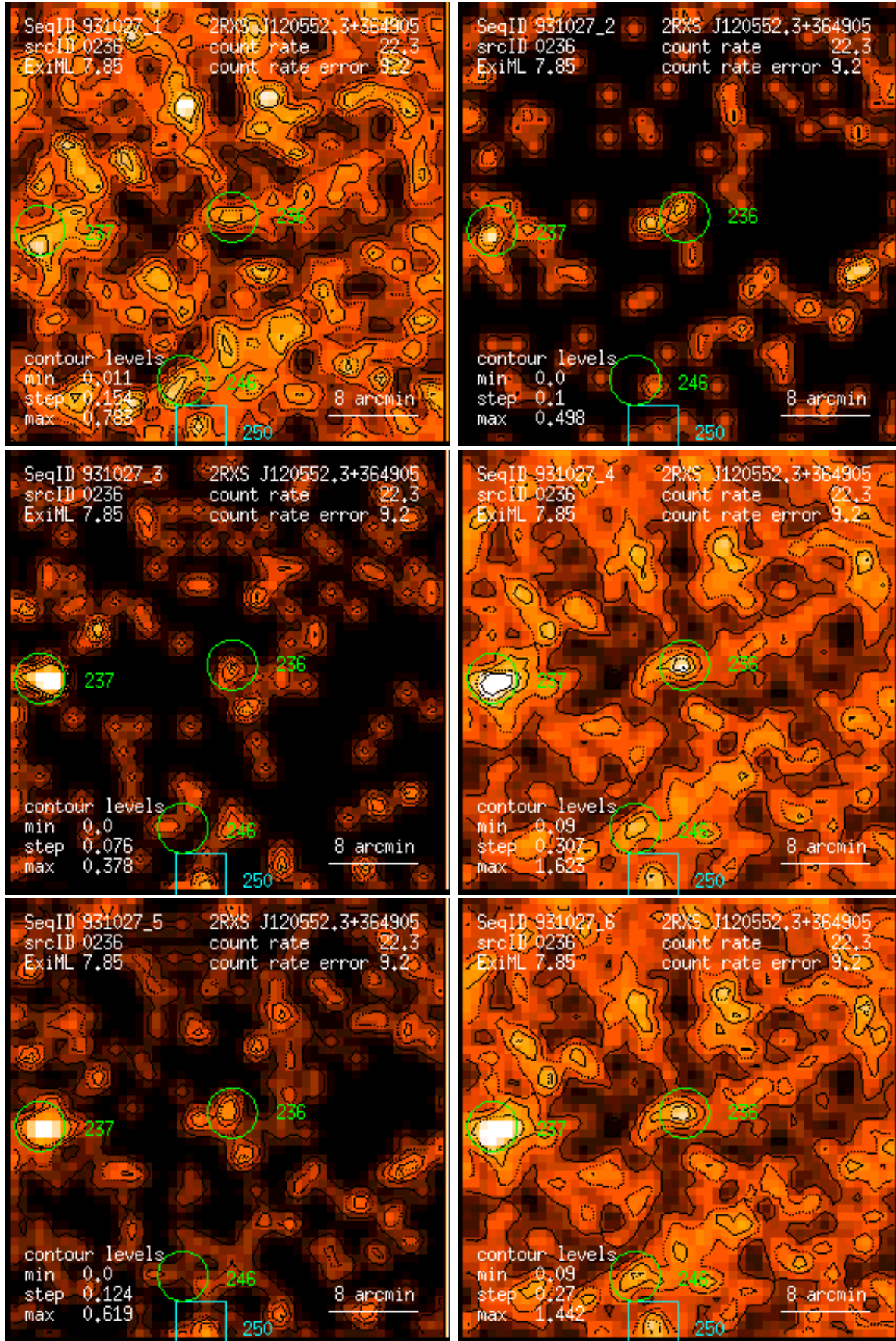
Figure 236: RASS 931027: detection 0236: band rate images, Gaussian filter: (1) PSPC channels 11 – 41, (2) 52 – 90, (3) 91 – 201, (4) 11 – 235, (5) 52 – 201, (6) 11 – 201. Broad band rates in counts/ks. Band rate contour levels in counts/ks/arcmin 2 .
