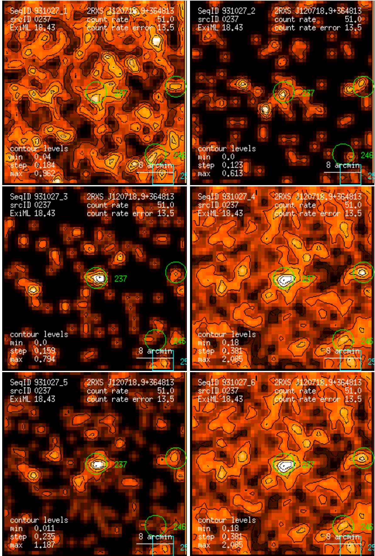
Figure 237: RASS 931027: detection 0237: band rate images, Gaussian filter: (1) PSPC channels 11 – 41, (2) 52 – 90, (3) 91 – 201, (4) 11 – 235, (5) 52 – 201, (6) 11 – 201. Broad band rates in counts/ks. Band rate contour levels in counts/ks/arcmin 2 .
