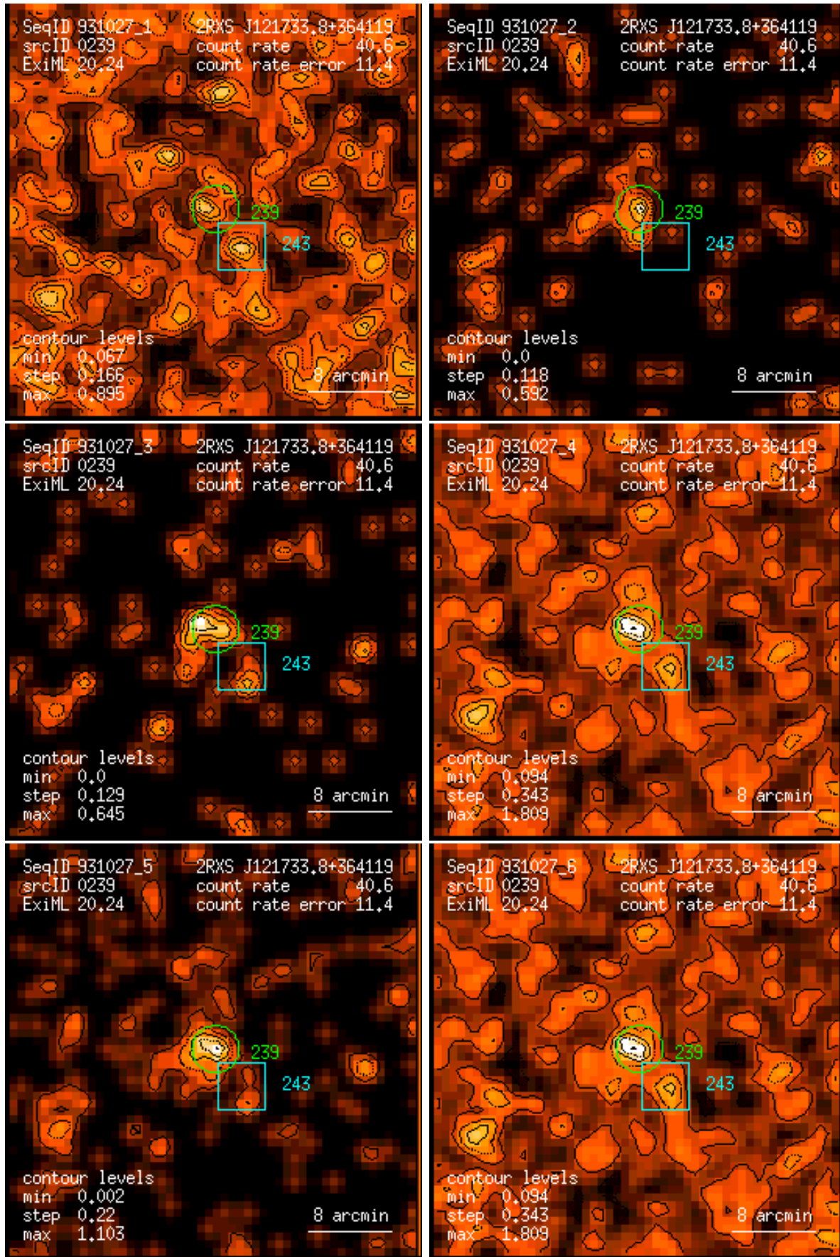
Figure 239: RASS 931027: detection 0239: band rate images, Gaussian filter: (1) PSPC channels 11 – 41, (2) 52 – 90, (3) 91 – 201, (4) 11 – 235, (5) 52 – 201, (6) 11 – 201. Broad band rates in counts/ks. Band rate contour levels in counts/ks/arcmin 2 .
