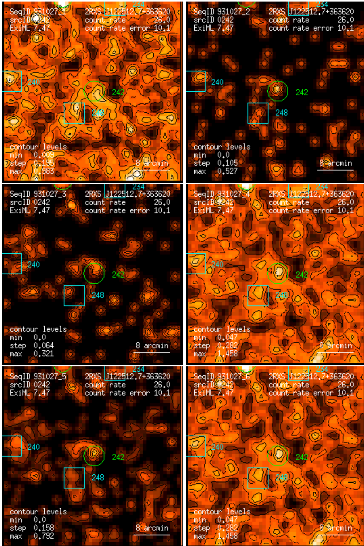
Figure 242: RASS 931027: detection 0242: band rate images, Gaussian filter: (1) PSPC channels 11 – 41, (2) 52 – 90, (3) 91 – 201, (4) 11 – 235, (5) 52 – 201, (6) 11 – 201. Broad band rates in counts/ks. Band rate contour levels in counts/ks/arcmin 2 .
