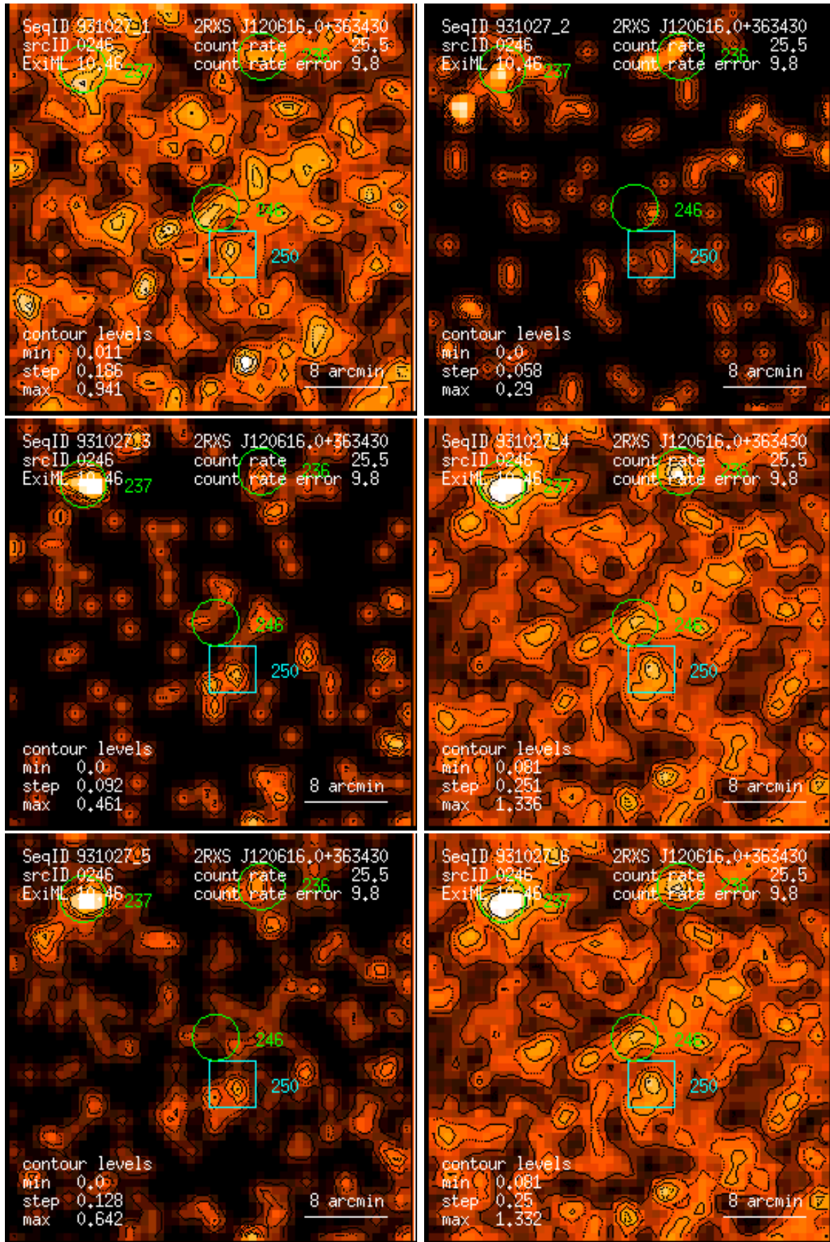
Figure 246: RASS 931027: detection 0246: band rate images, Gaussian filter: (1) PSPC channels 11 – 41, (2) 52 – 90, (3) 91 – 201, (4) 11 – 235, (5) 52 – 201, (6) 11 – 201. Broad band rates in counts/ks. Band rate contour levels in counts/ks/arcmin 2 .
