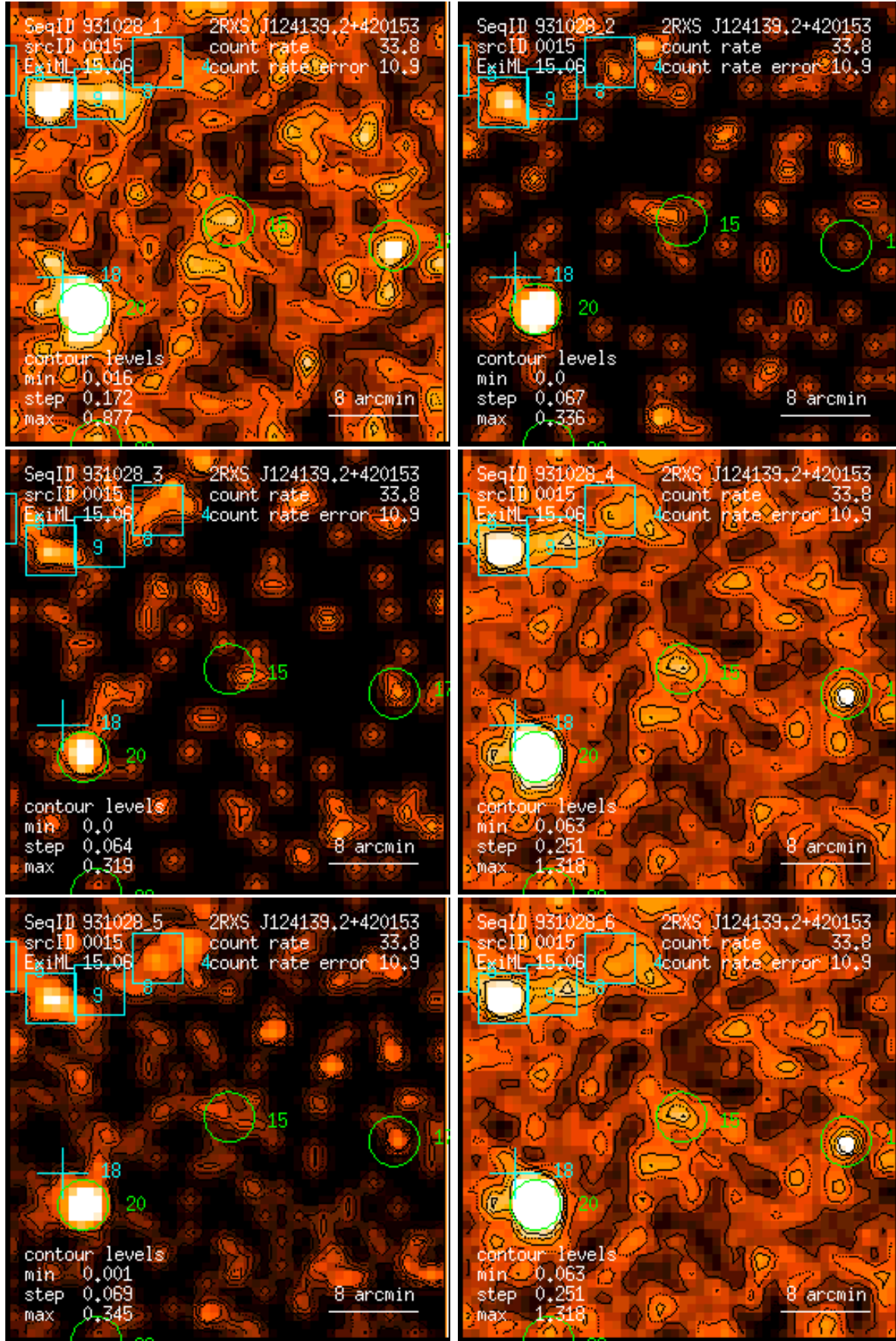
Figure 15: RASS 931028: detection 0015: band rate images, Gaussian filter: (1) PSPC channels 11 – 41, (2) 52 – 90, (3) 91 – 201, (4) 11 – 235, (5) 52 – 201, (6) 11 – 201. Broad band rates in counts/ks. Band rate contour levels in counts/ks/arcmin 2 .
