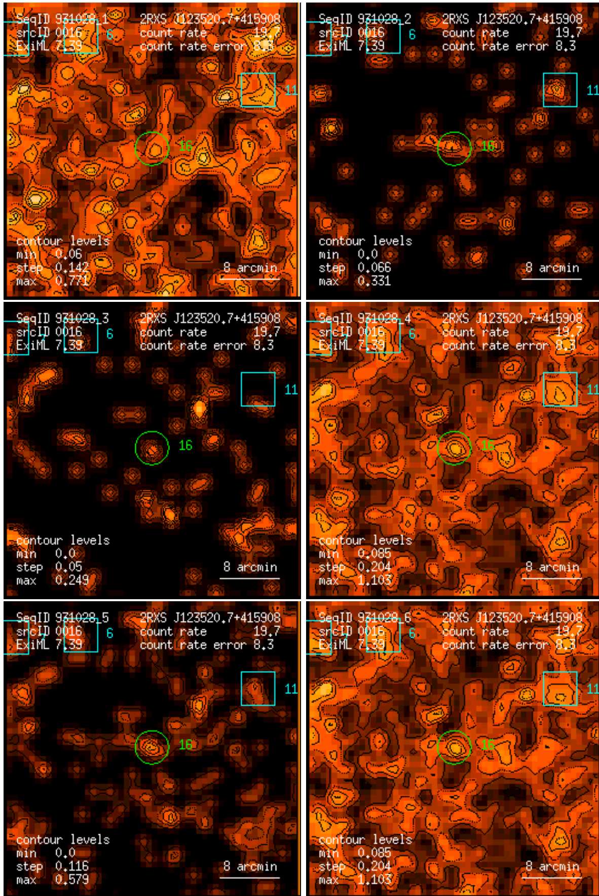
Figure 16: RASS 931028: detection 0016: band rate images, Gaussian filter: (1) PSPC channels 11 – 41, (2) 52 – 90, (3) 91 – 201, (4) 11 – 235, (5) 52 – 201, (6) 11 – 201. Broad band rates in counts/ks. Band rate contour levels in counts/ks/arcmin 2 .
