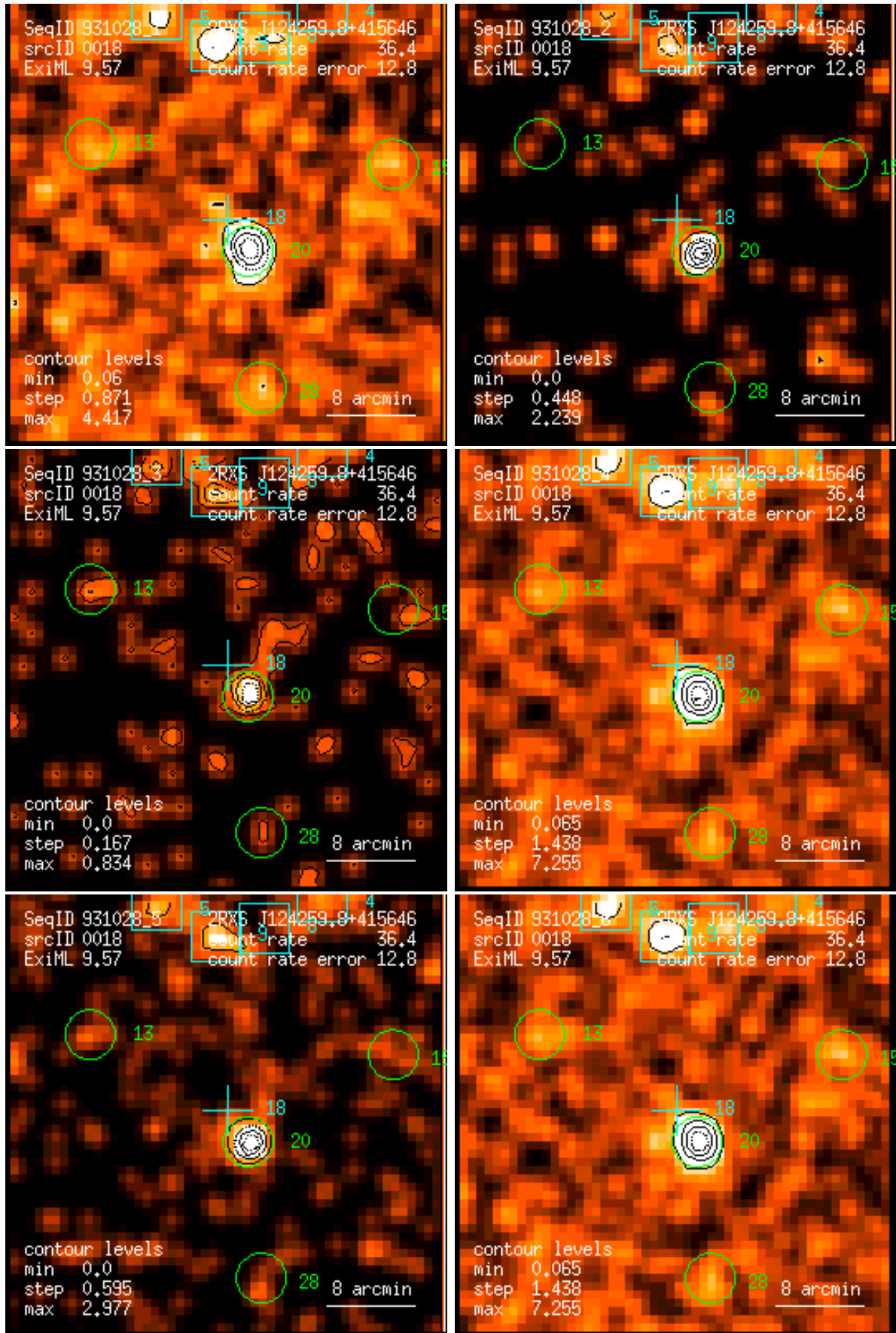
Figure 18: RASS 931028: detection 0018: band rate images, Gaussian filter: (1) PSPC channels 11 – 41, (2) 52 – 90, (3) 91 – 201, (4) 11 – 235, (5) 52 – 201, (6) 11 – 201. Broad band rates in counts/ks. Band rate contour levels in counts/ks/arcmin 2 .
