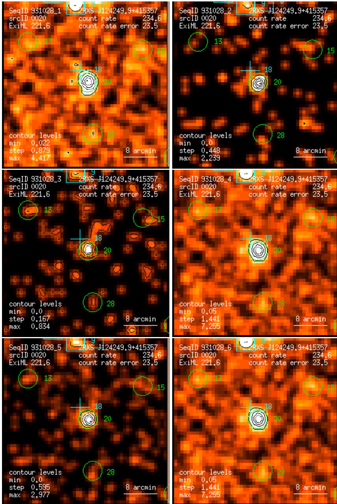
Figure 20: RASS 931028: detection 0020: band rate images, Gaussian filter: (1) PSPC channels 11 – 41, (2) 52 – 90, (3) 91 – 201, (4) 11 – 235, (5) 52 – 201, (6) 11 – 201. Broad band rates in counts/ks. Band rate contour levels in counts/ks/arcmin 2 .
