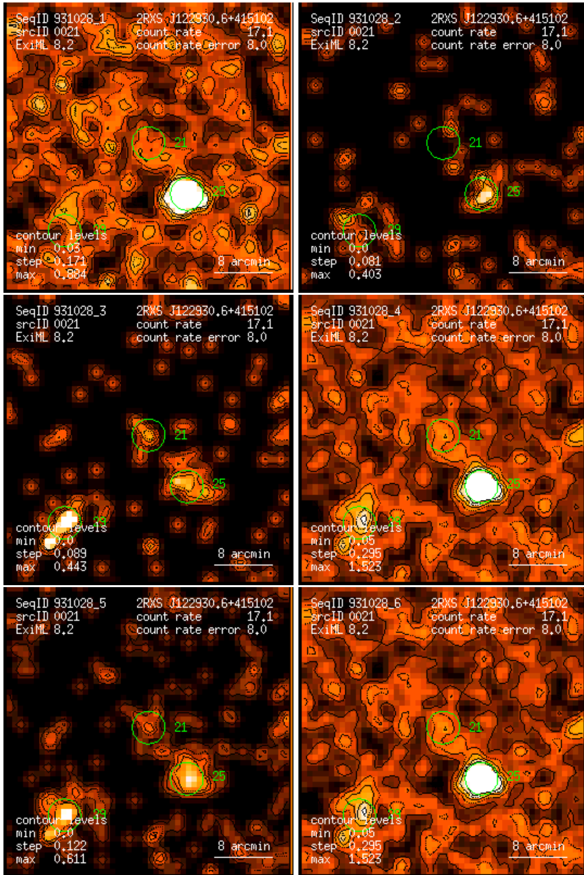
Figure 21: RASS 931028: detection 0021: band rate images, Gaussian filter: (1) PSPC channels 11 – 41, (2) 52 – 90, (3) 91 – 201, (4) 11 – 235, (5) 52 – 201, (6) 11 – 201. Broad band rates in counts/ks. Band rate contour levels in counts/ks/arcmin 2 .
