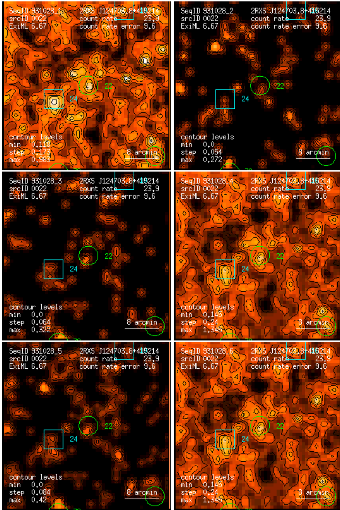
Figure 22: RASS 931028: detection 0022: band rate images, Gaussian filter: (1) PSPC channels 11 – 41, (2) 52 – 90, (3) 91 – 201, (4) 11 – 235, (5) 52 – 201, (6) 11 – 201. Broad band rates in counts/ks. Band rate contour levels in counts/ks/arcmin 2 .
